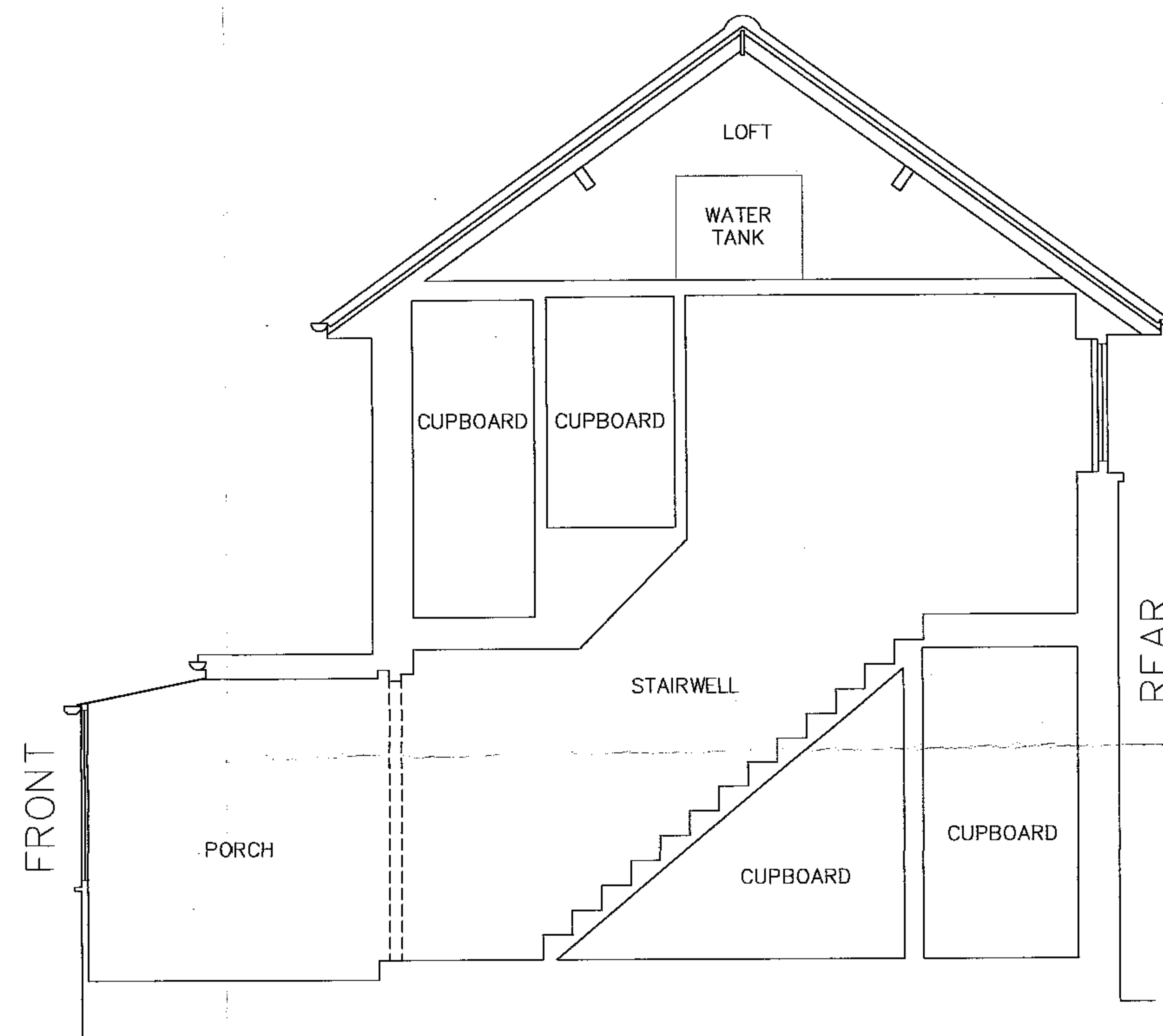
SECTION B-B
