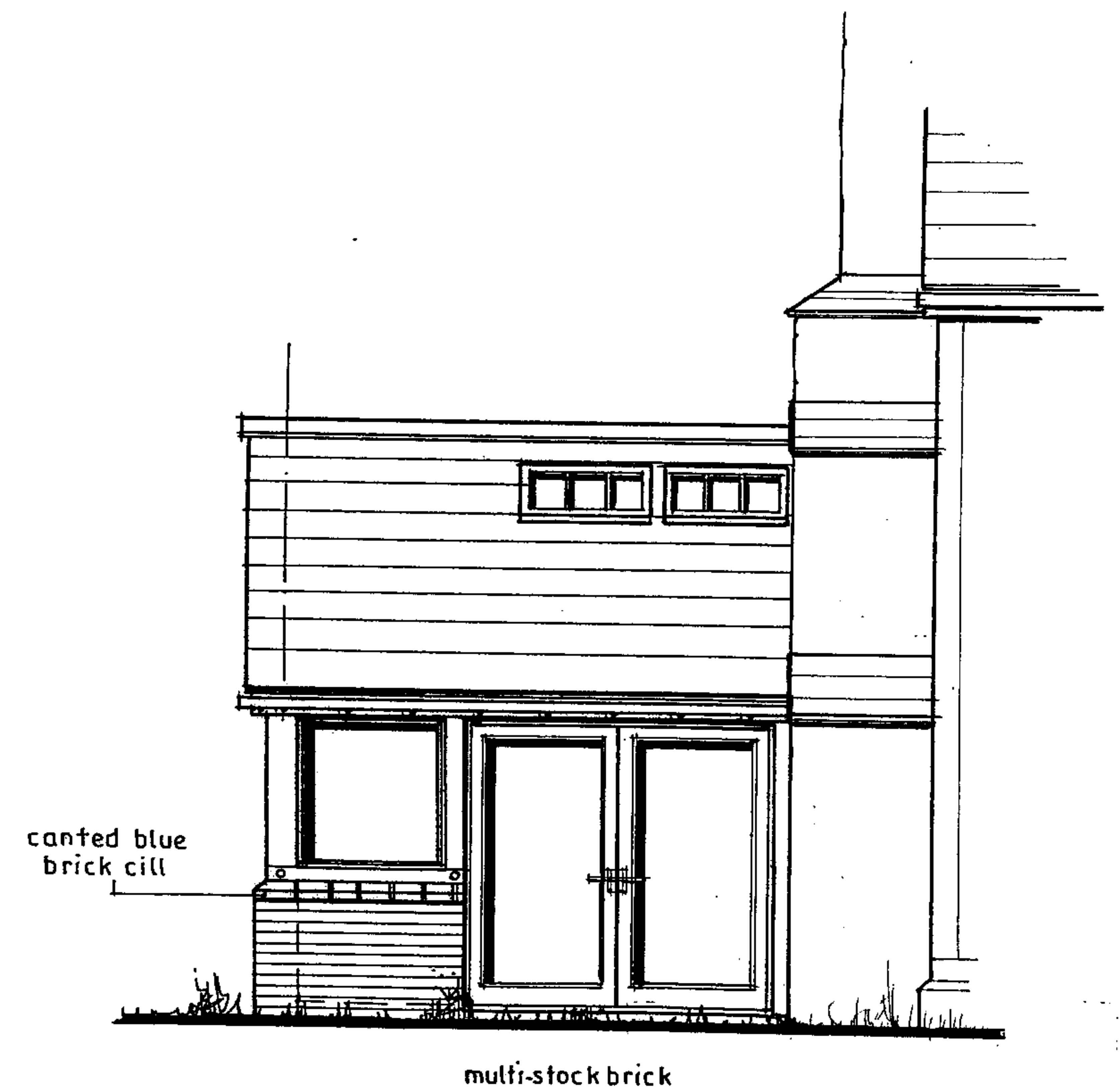
SIDE ELEVATION 1:50
