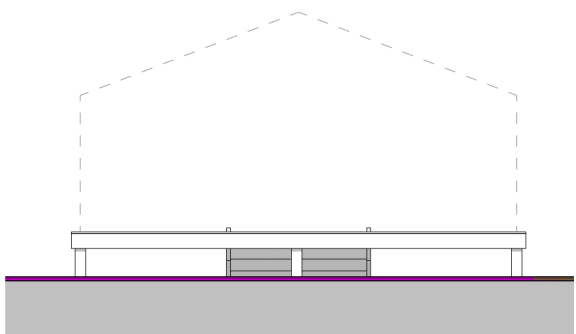
South East Elevation 1 : 100
