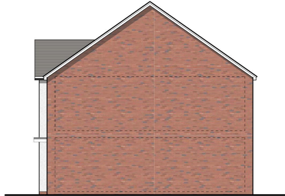
Gable Elevation Plot 34
