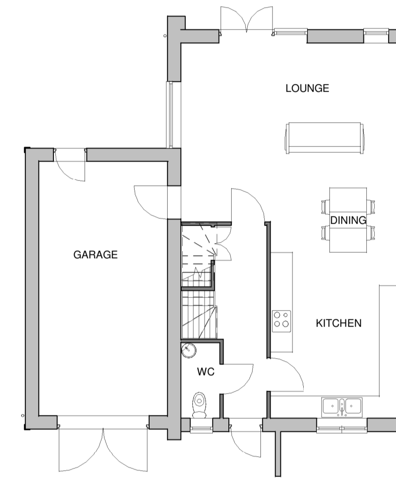
Ground floor plans- Plot 3 1 : 100
