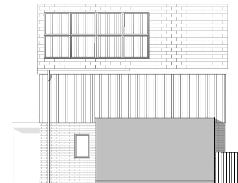
Plot 2- Eastern elevation 1 : 100
