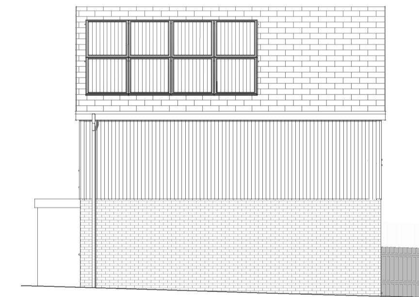
Plot 1- Eastern elevation 1 : 100
