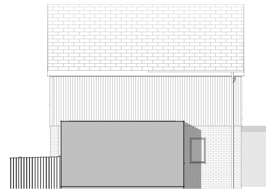
Plot 1- Western elevation 1 : 100
