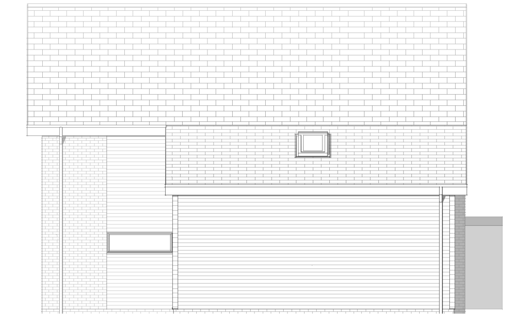
Plot 3- Western elevation 1 : 100
