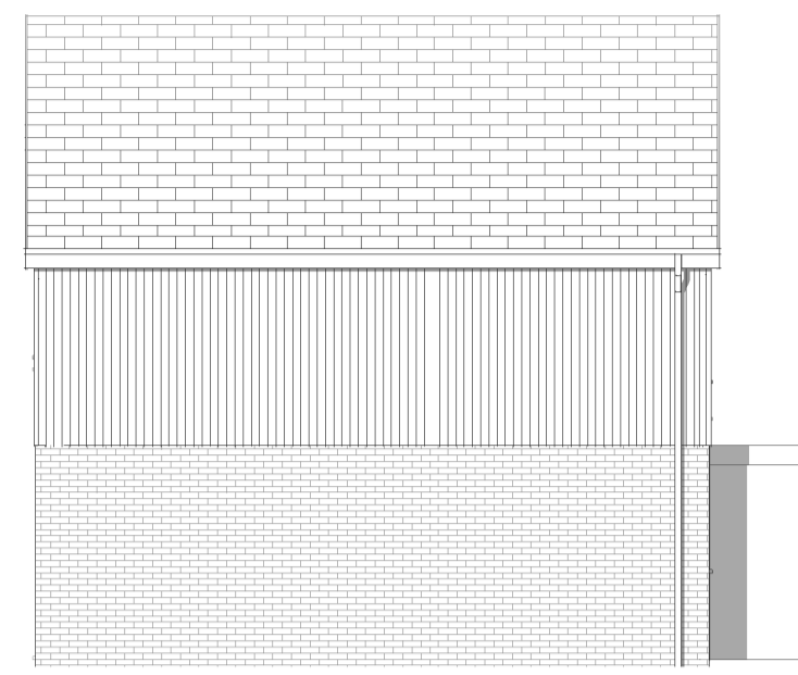
Plot 2- Western elevation 1 : 100
