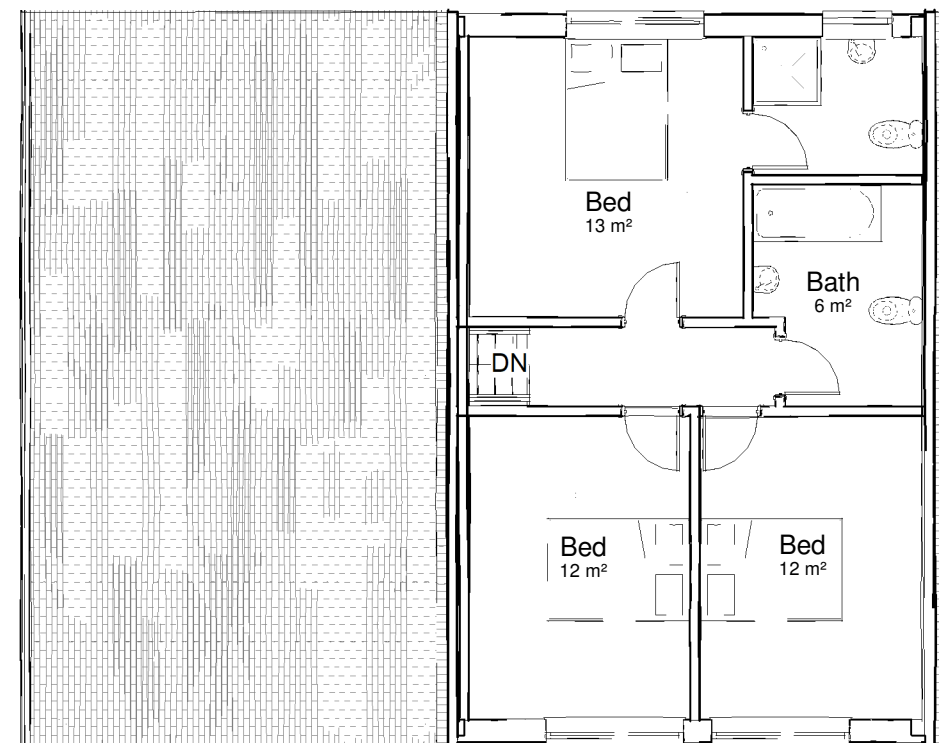
Barn C first floor plan 1 : 100
