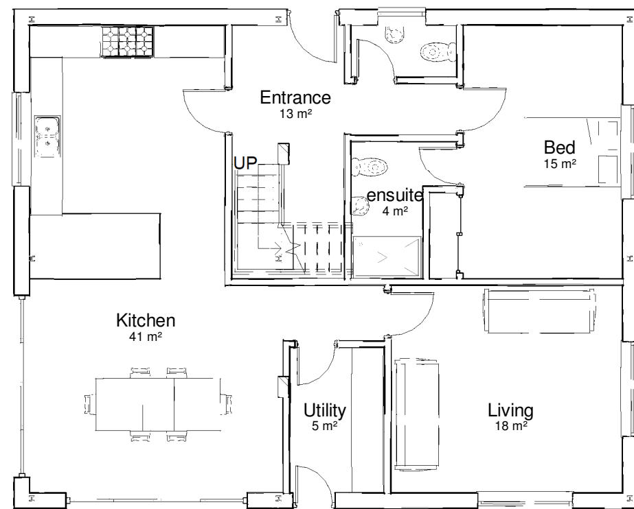
Barn C plan proposed 1 : 100
