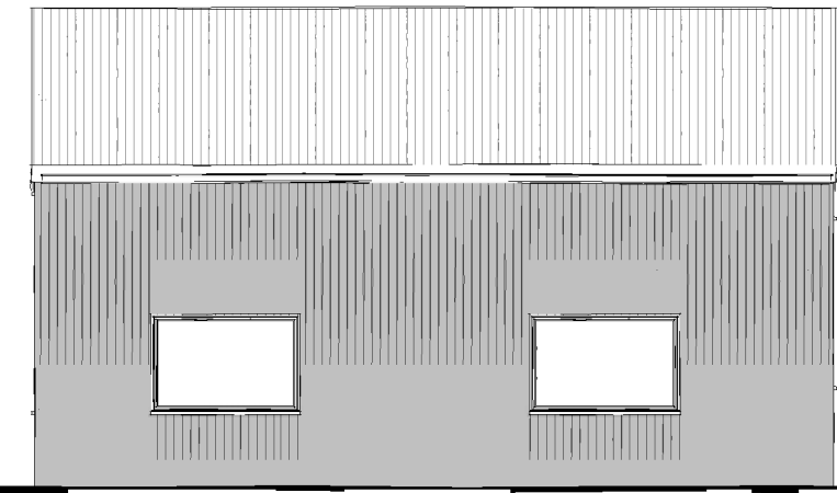
Barn C front proposed 1 : 100
