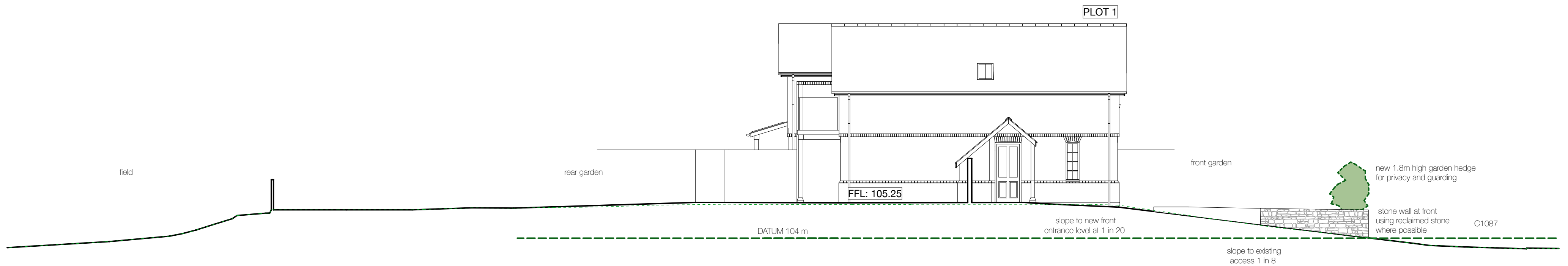
1. Proposed Site Cross section Plot 1
