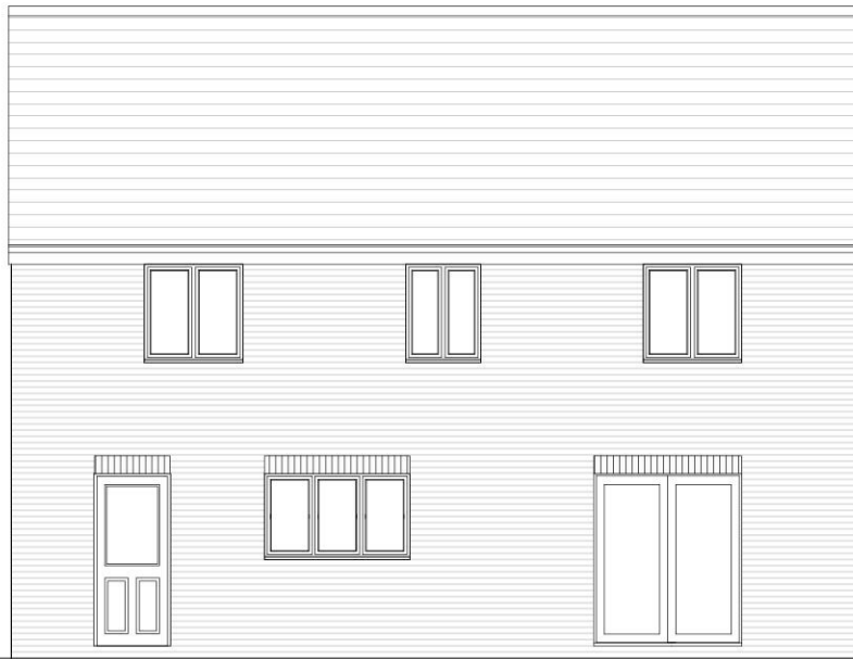
Rear Elevation
