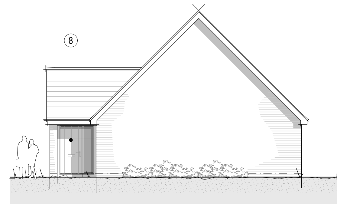
Side / Entrance Elevation
