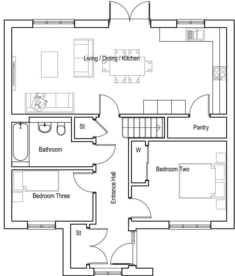
Ground Floor House Type C1
