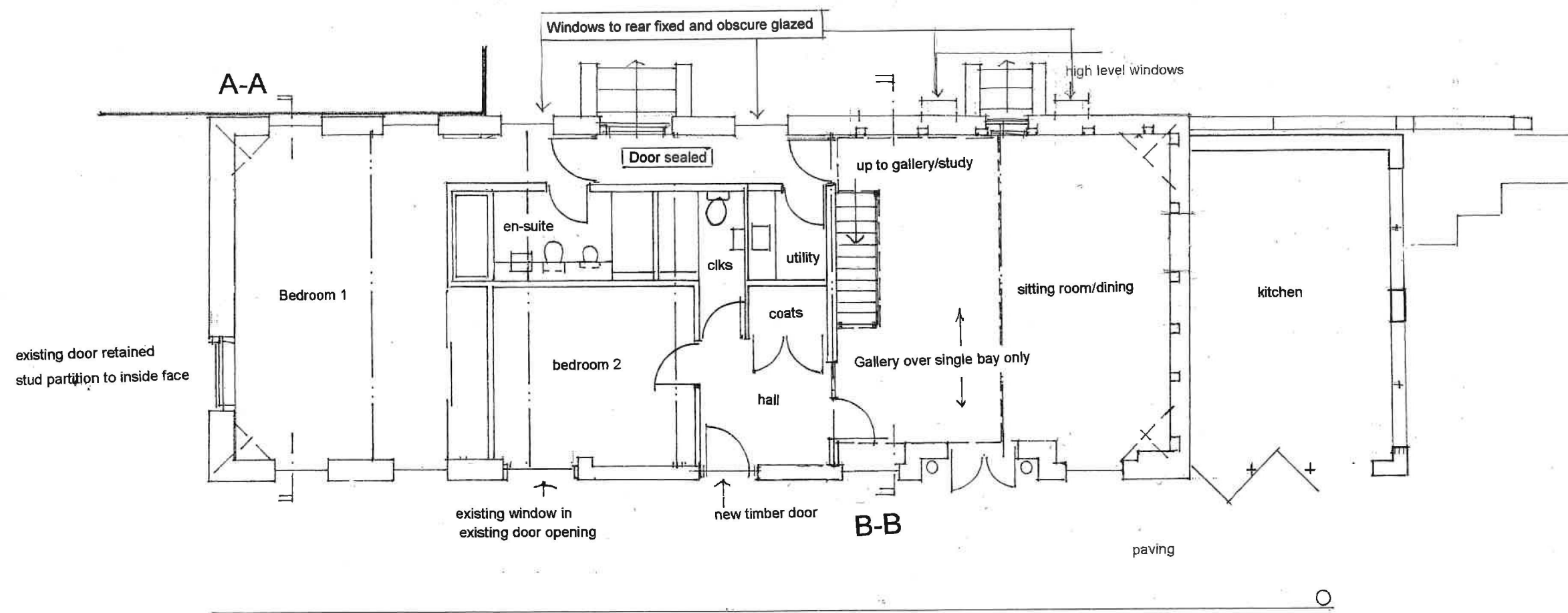
FLOOR PLAN
