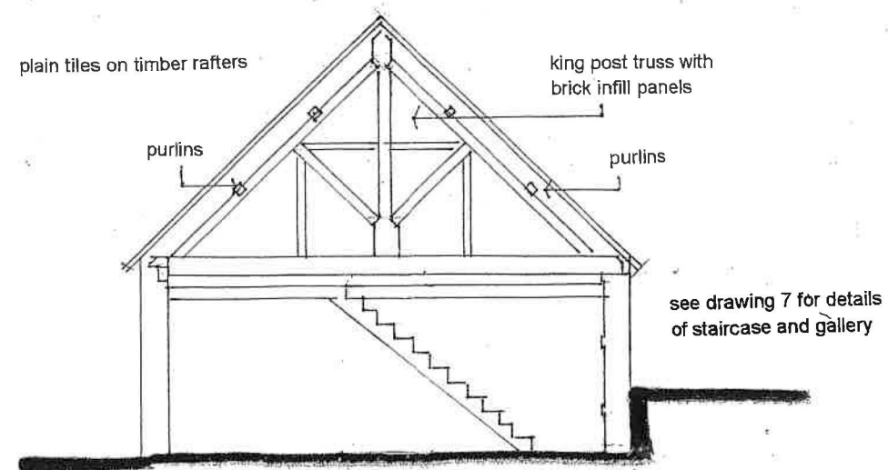
SECTION B-B
