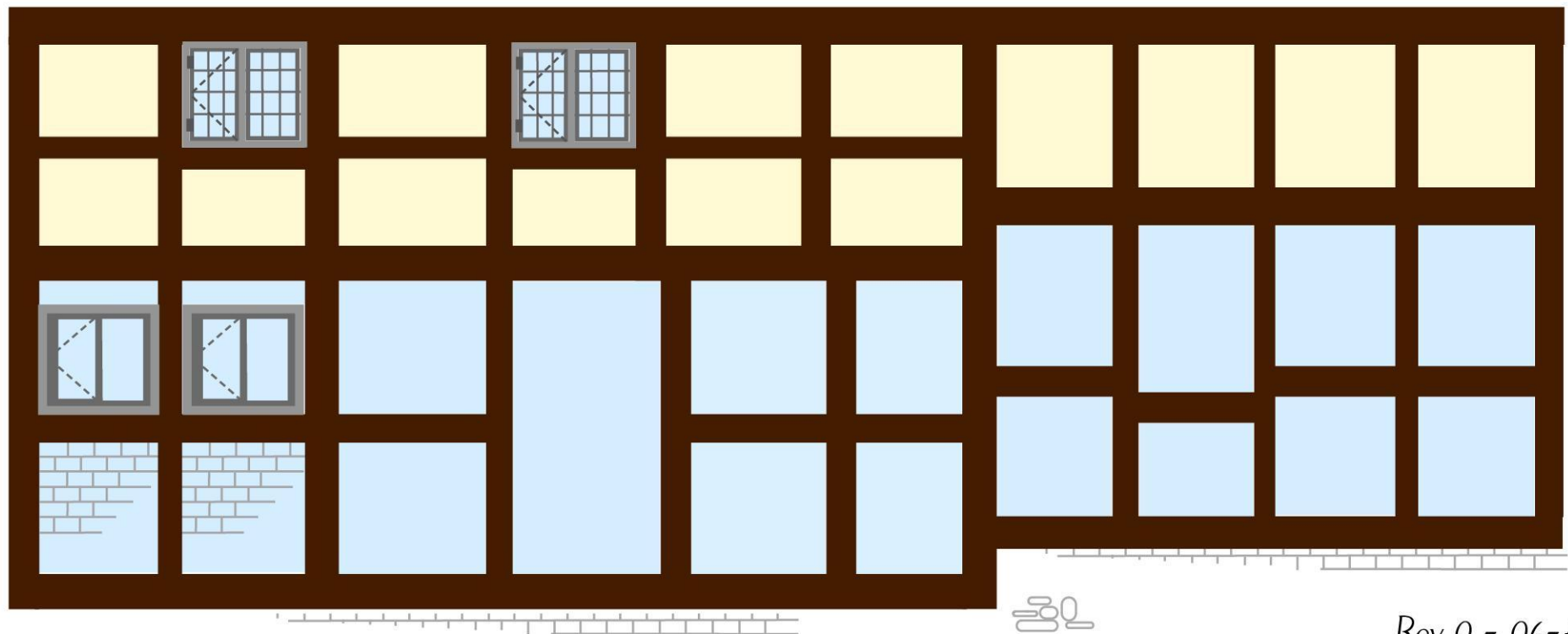
West Elevation
