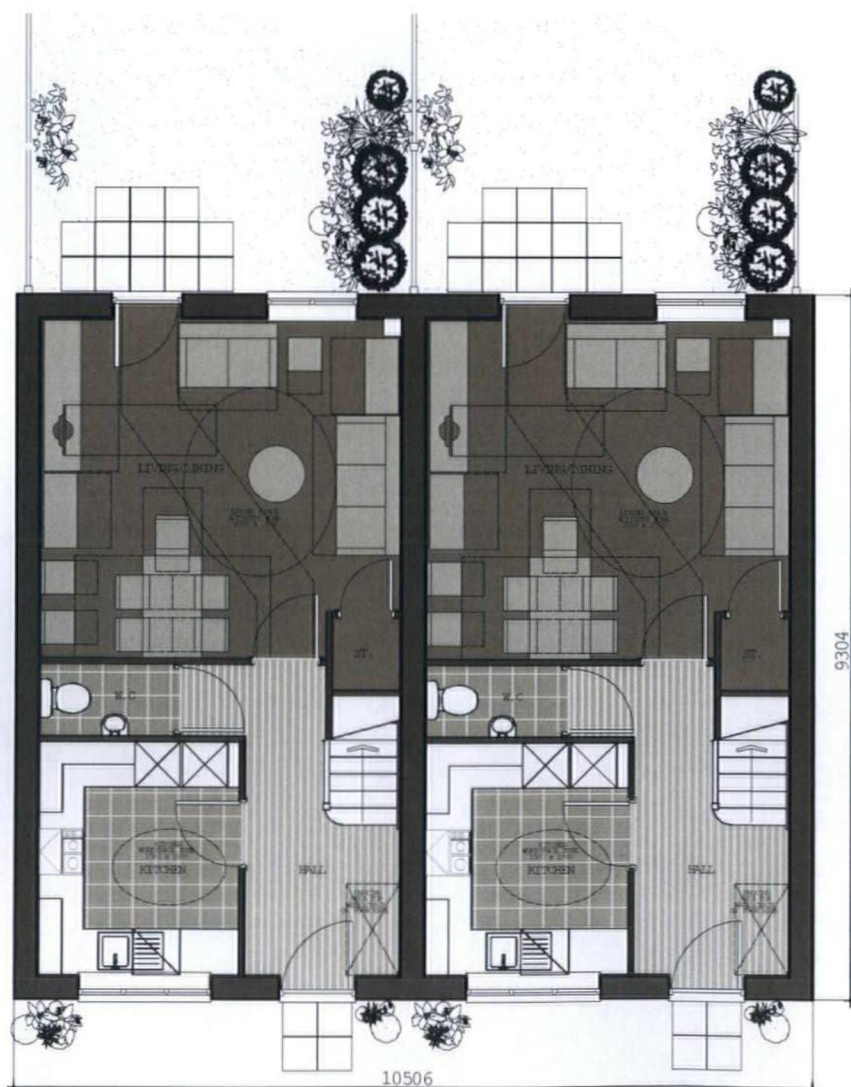
PLOTS 6 & 182 GROUND FLOOR PLAN
