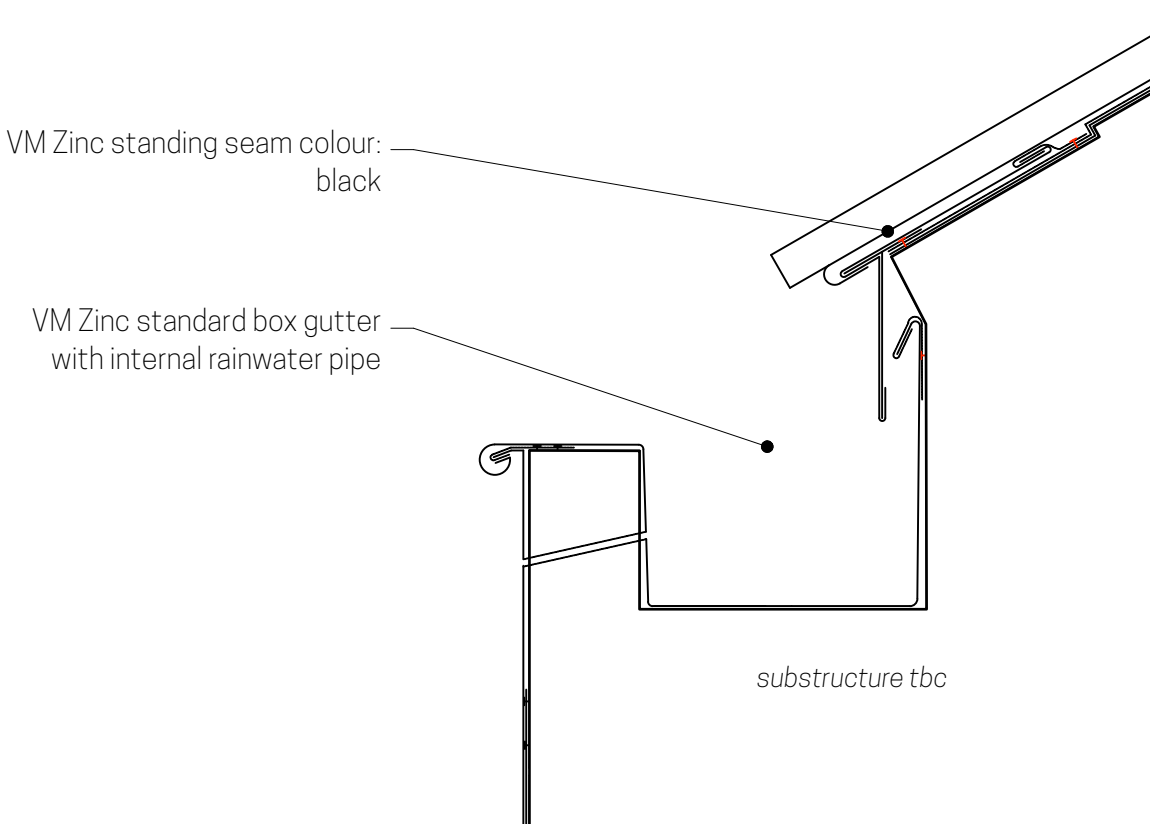
BOX GUTTER TO LEAN TO GARAGE
