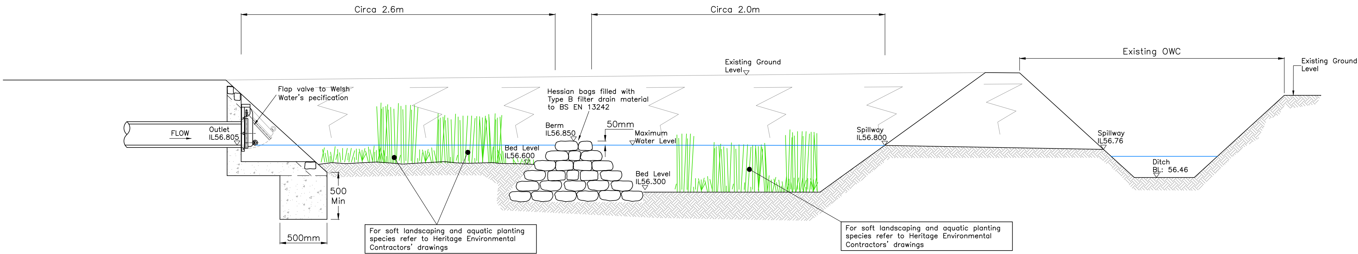
Section Through Wetland / Pond Scale 1:25
