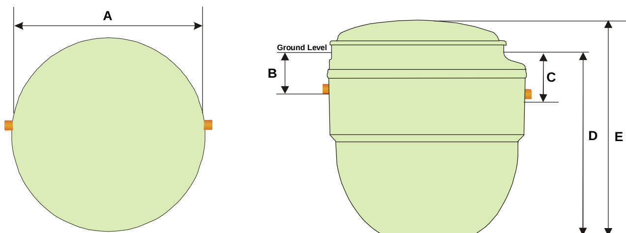
Fig. 1 General Dimensions
