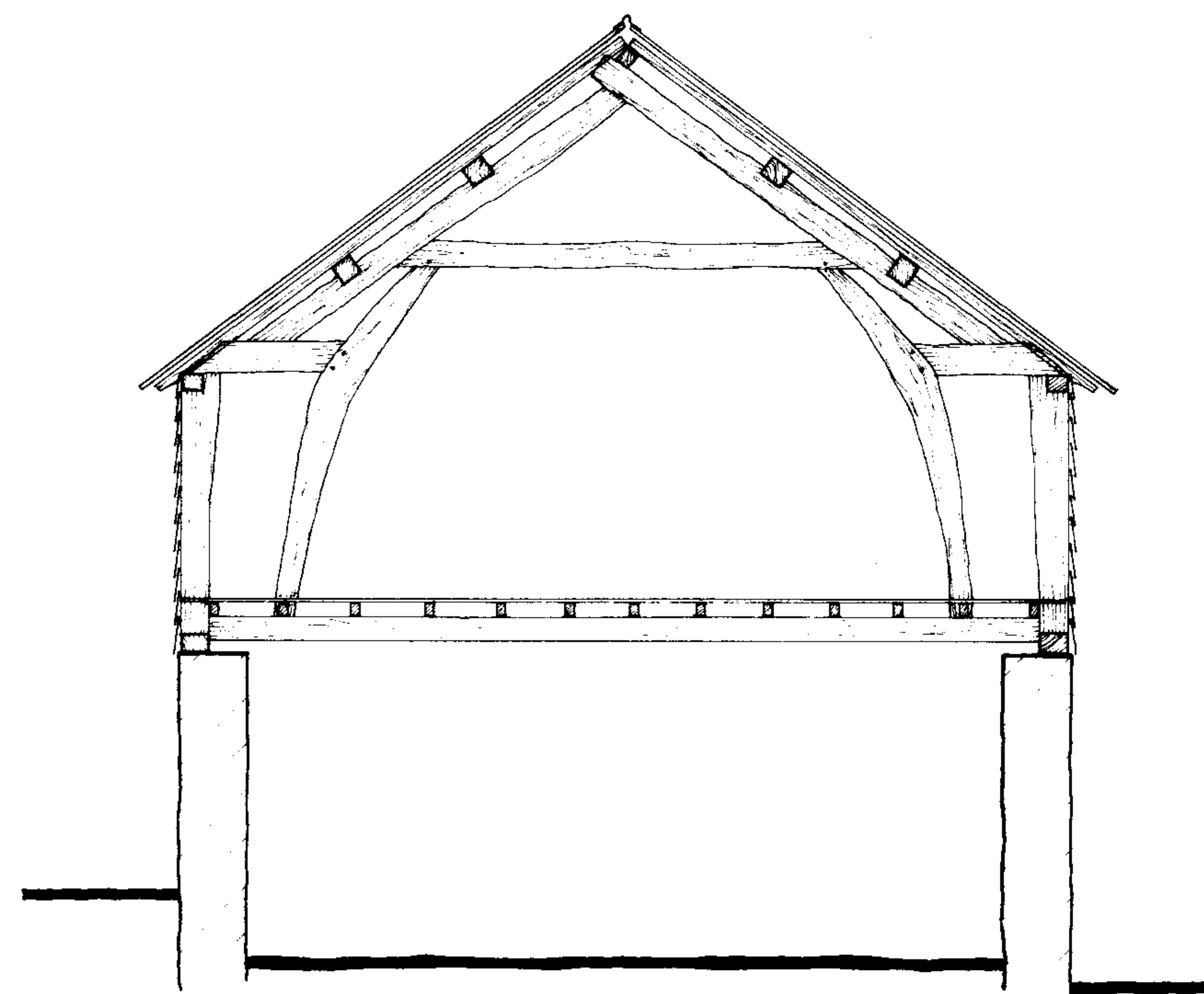
Section U - U
