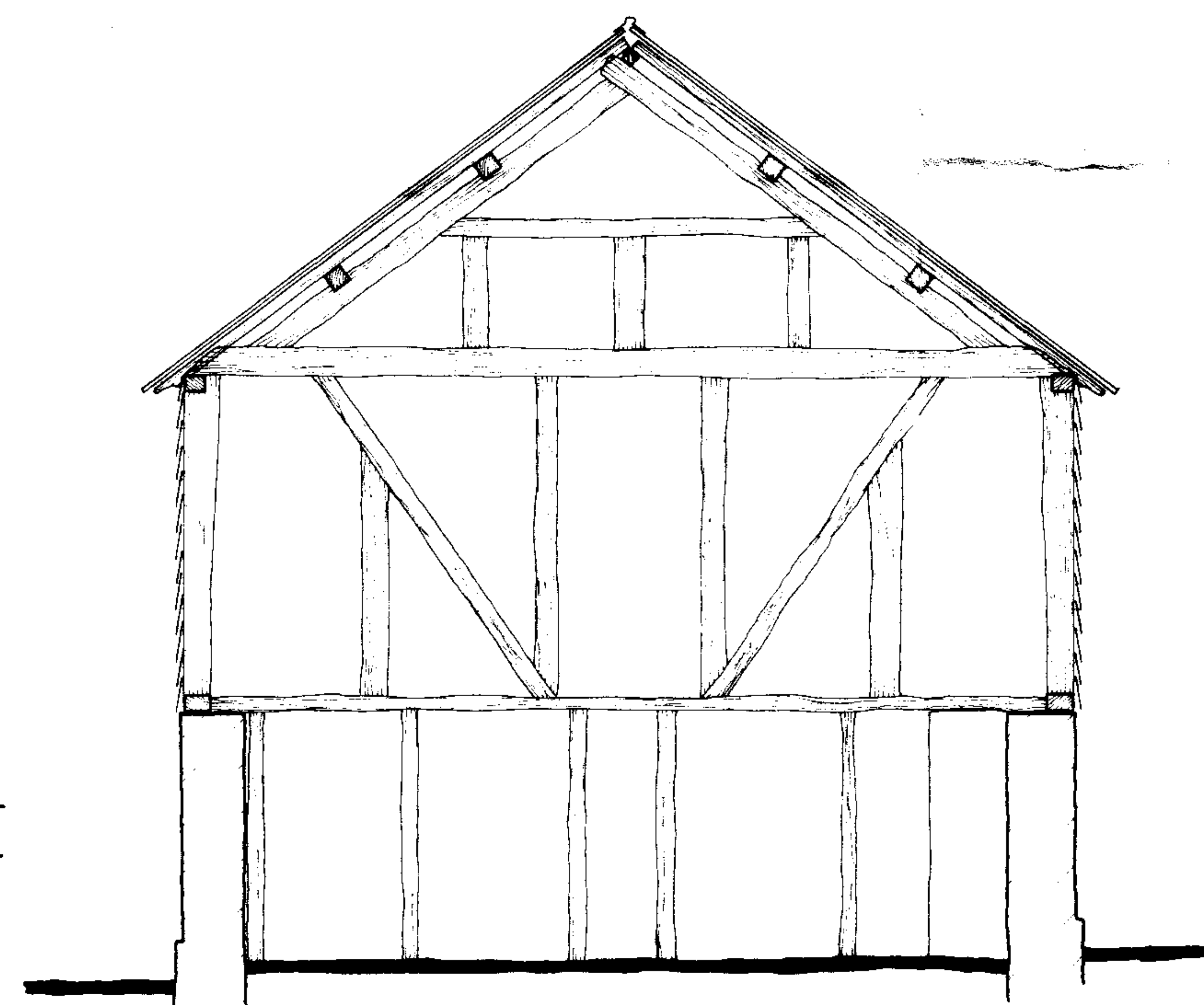
Section T - T
