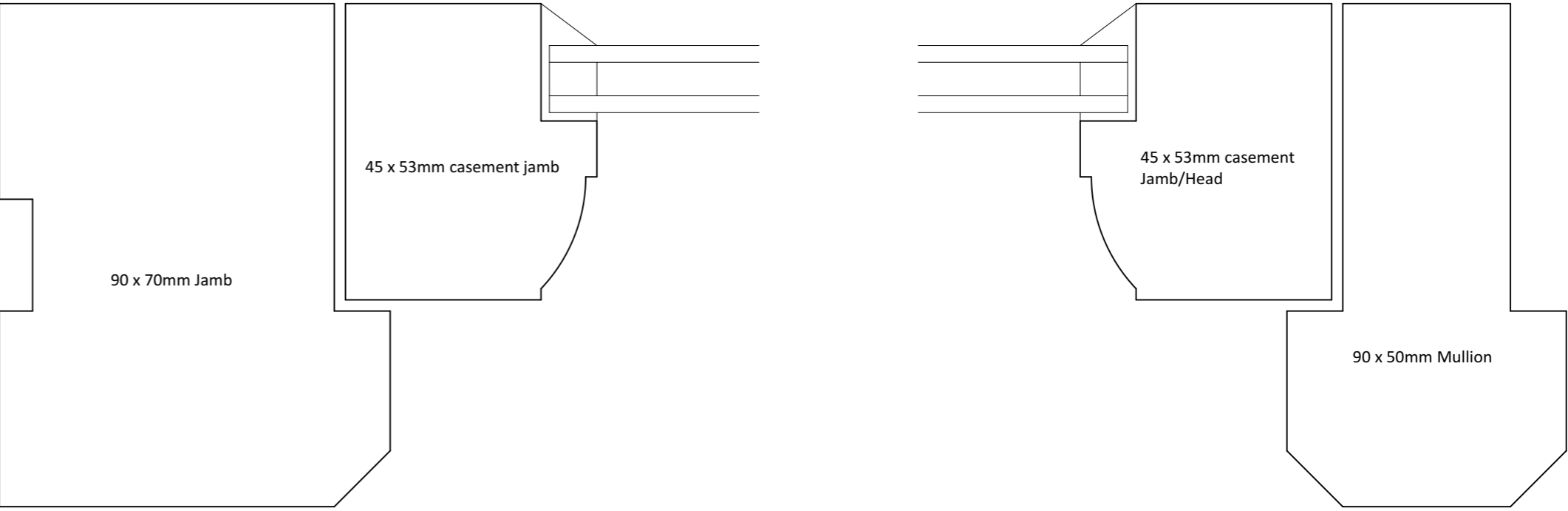
Full Size Horizontal Section
