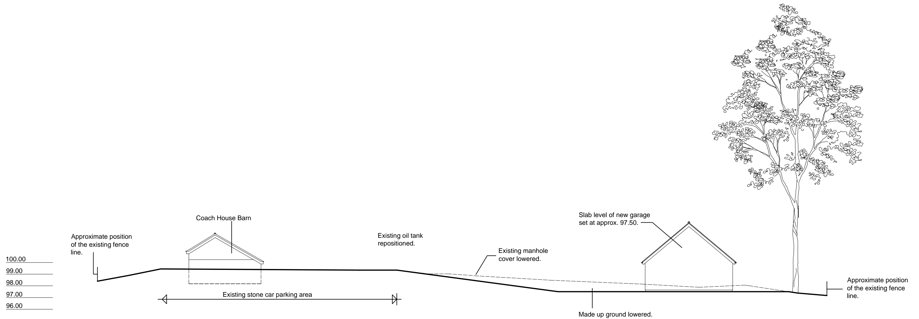
PROPOSED SECTION
