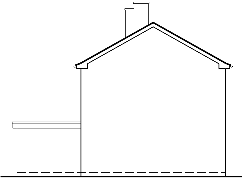
NORTH ELEVATION
