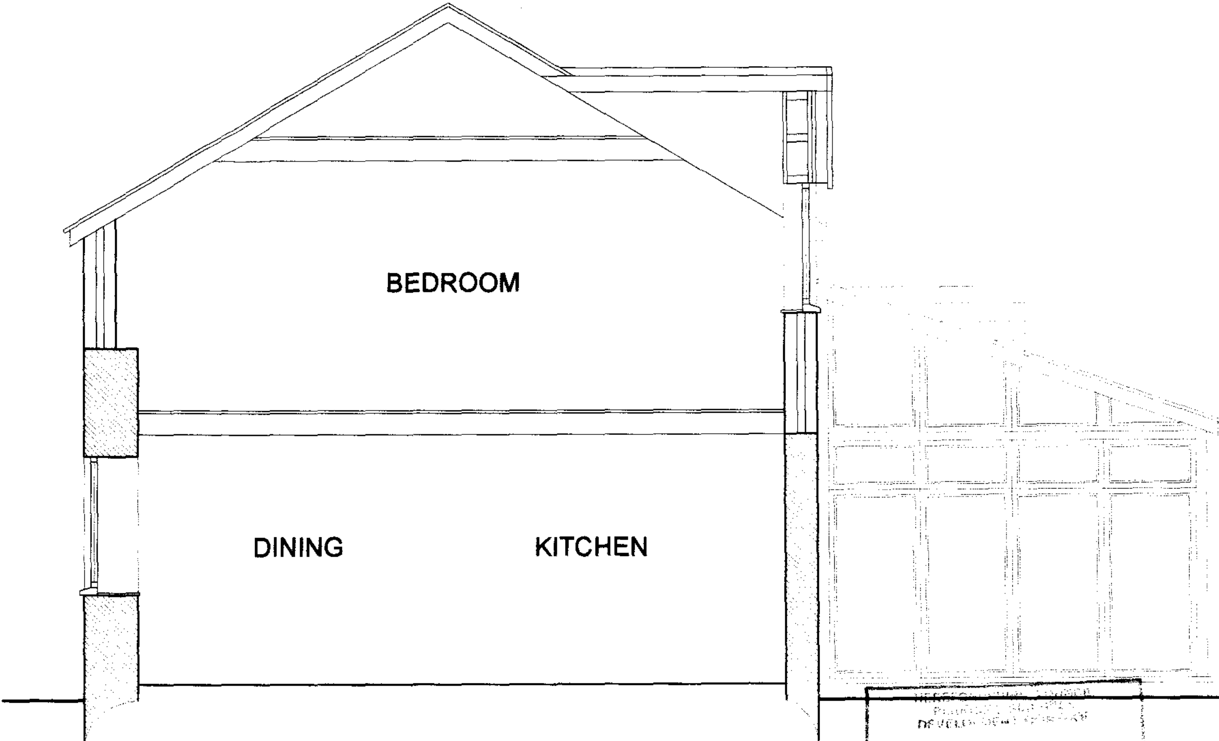
SECTION AS PROPOSED 1:50
