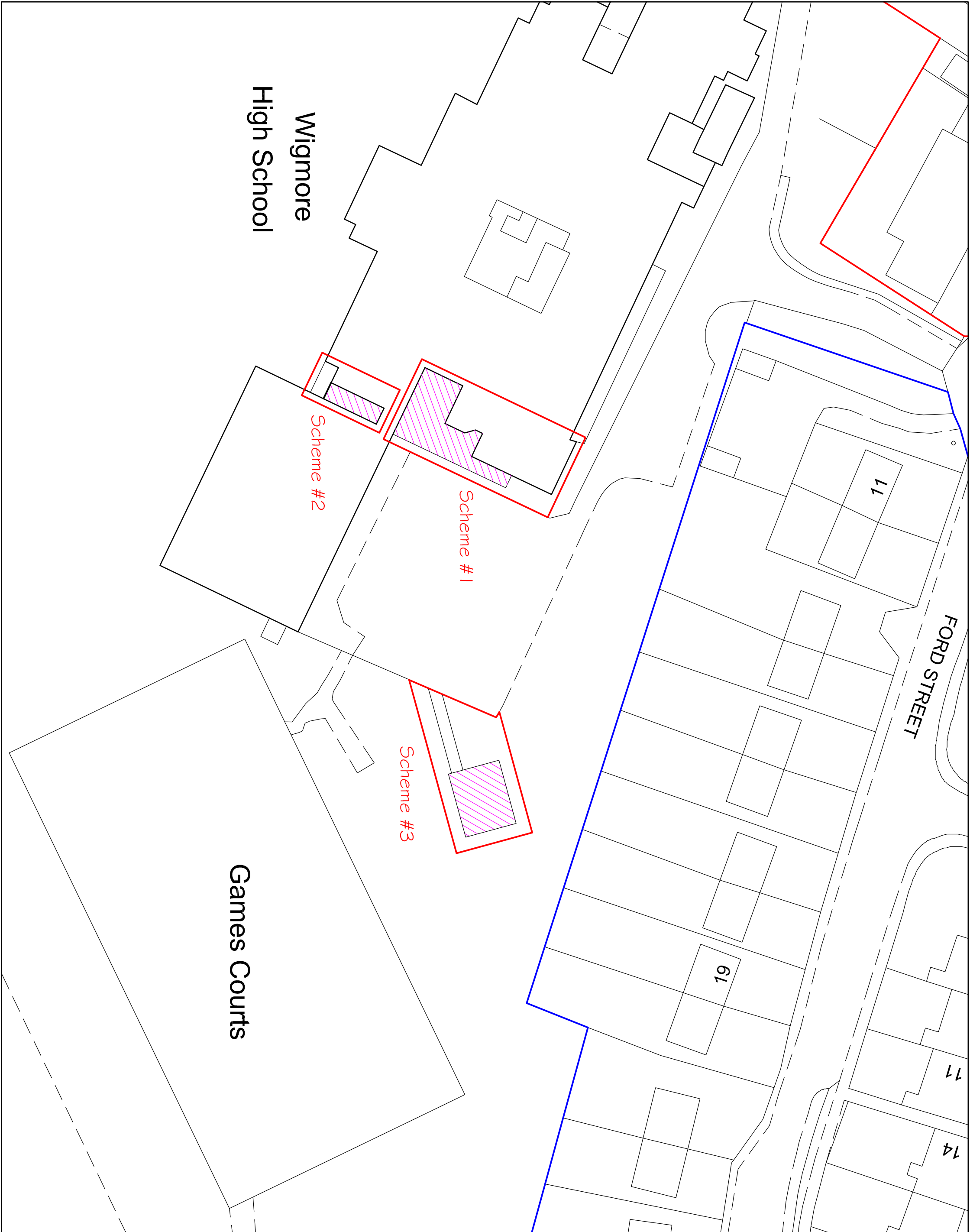
PROPOSED BLOCK PLAN SCALE 1 : 500
