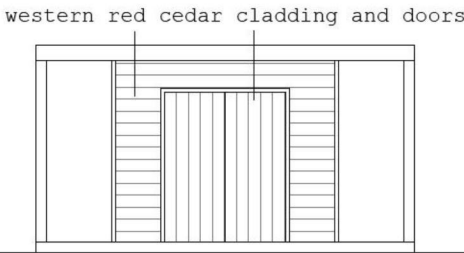
1:100 East Elevation
