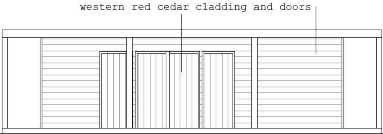
1:100 Riverside Elevation
