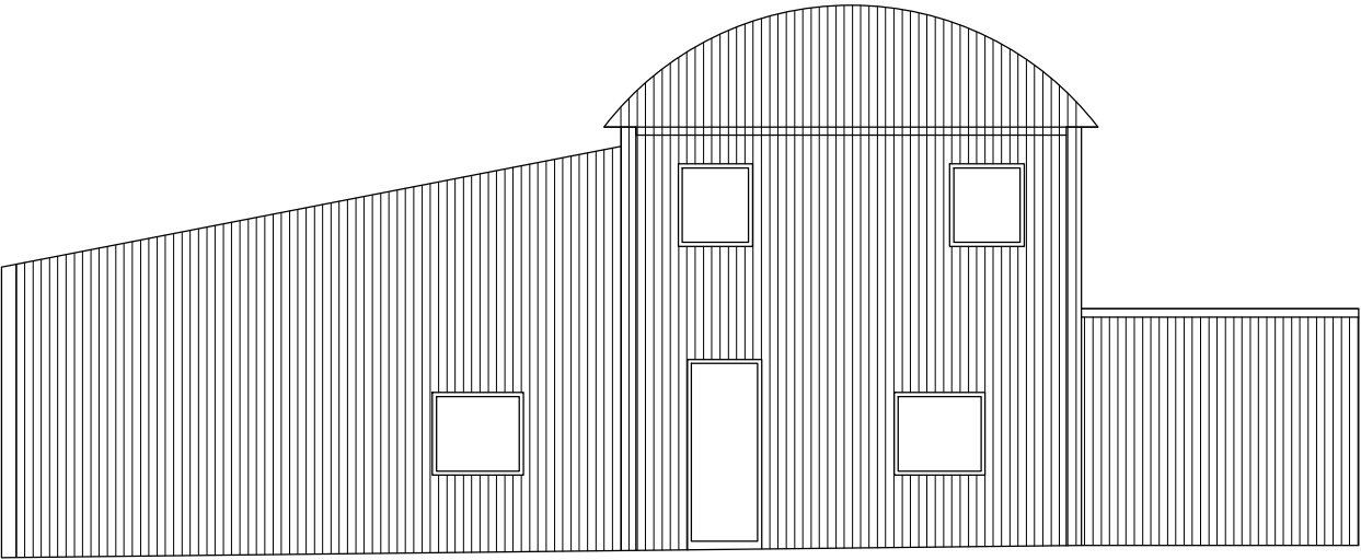
C - North Elevation
