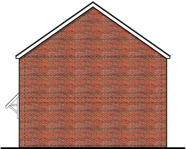
Plot 31 Side Elevation
