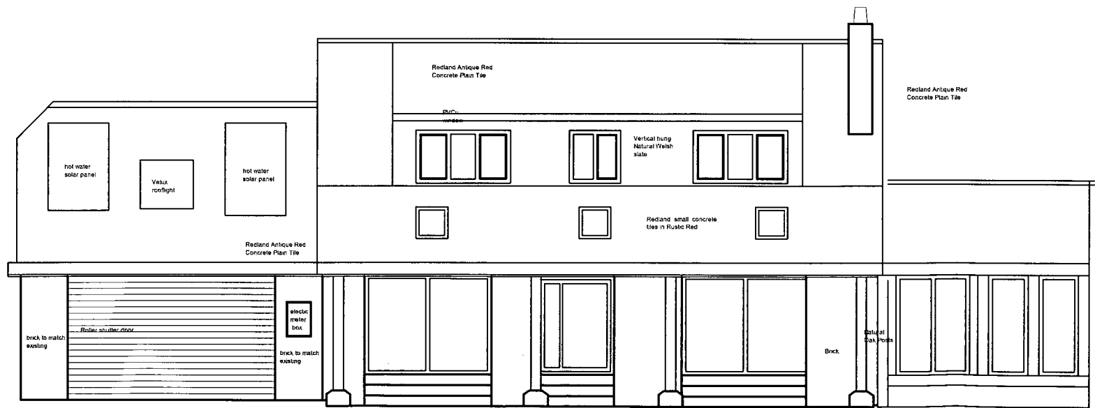
SOUTH ELEVATION
