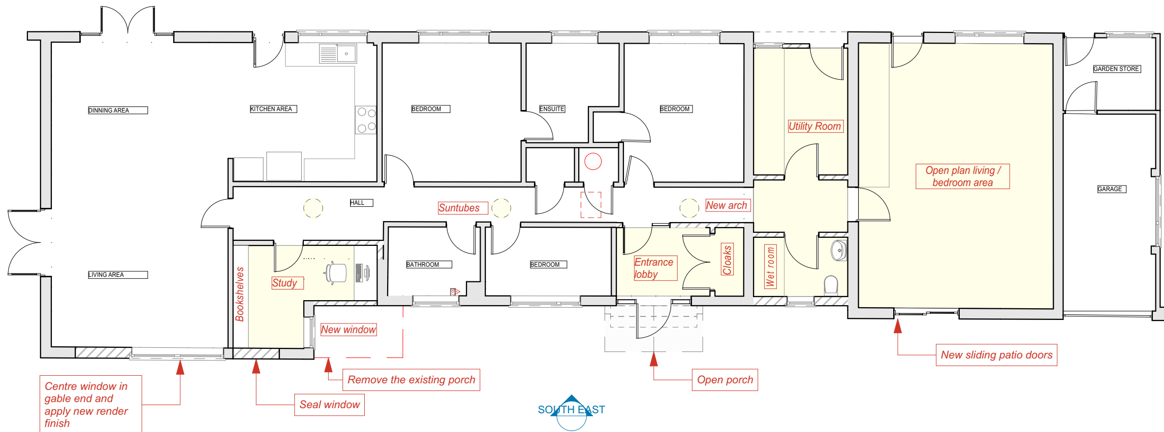
1 1:100 GROUND FLOOR AS PROPOSED
