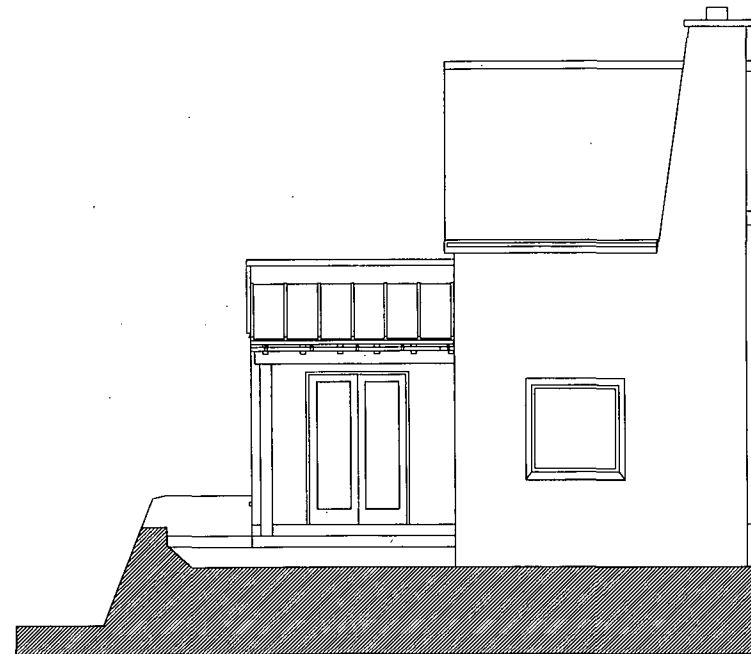
4. NORTH FRONT ELEVATION
