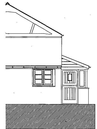
7. PORCH WEST ELEVATION
