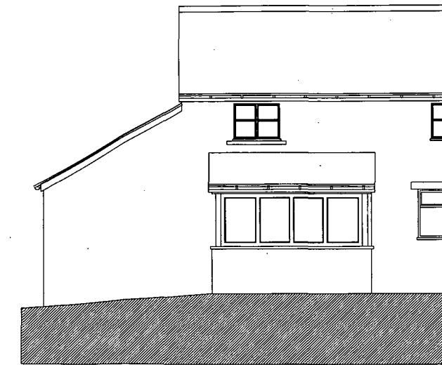
5. PORCH SOUTH ELEVATION
