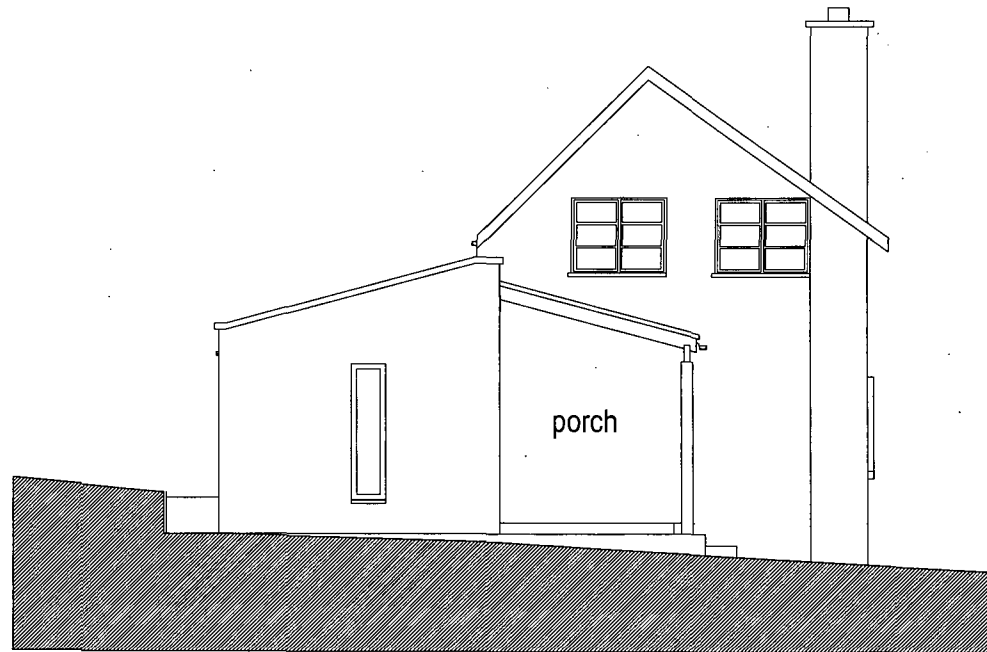
2. SIDE EAST ELEVATION
