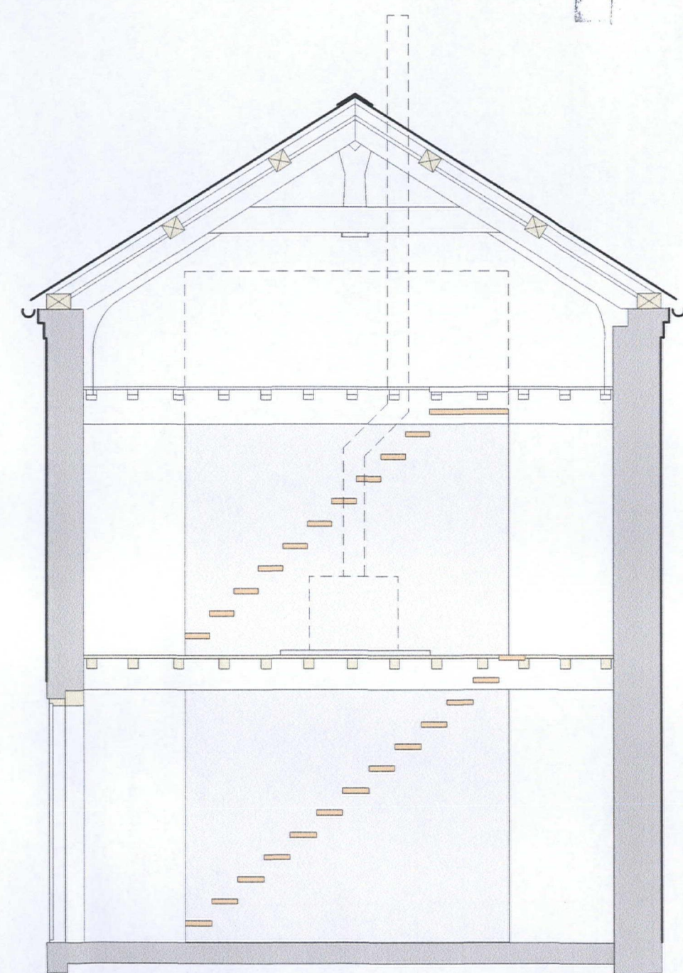
SECTION 1:50
