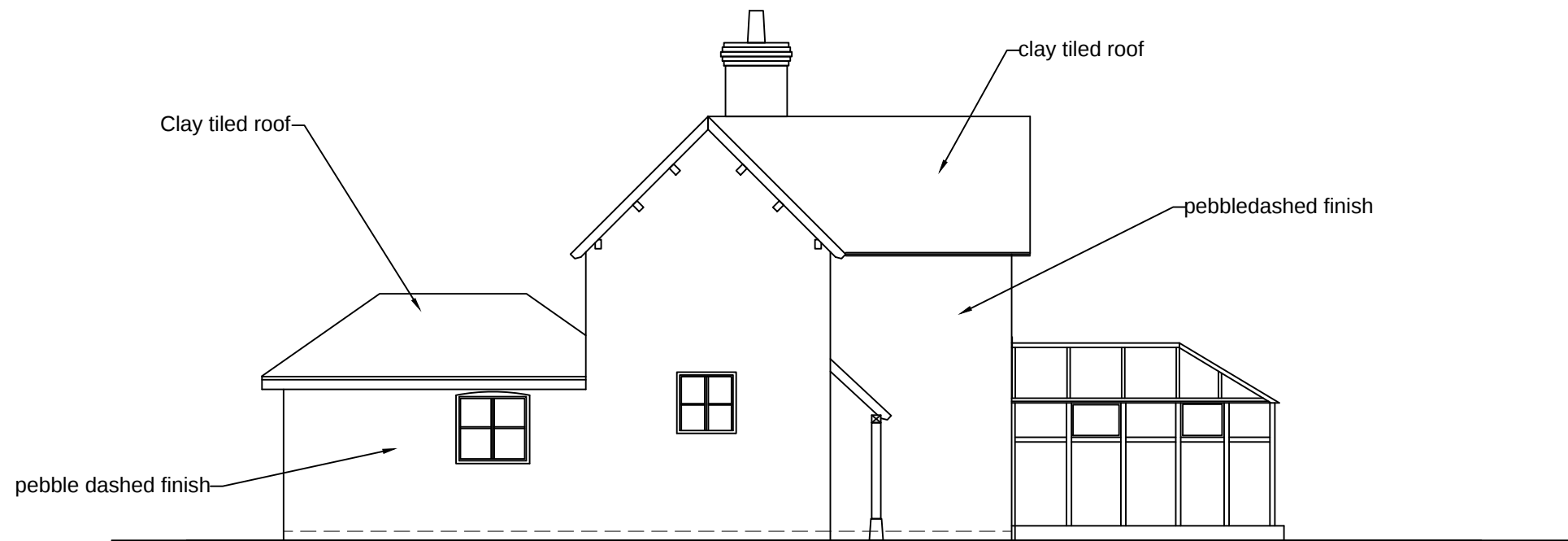
SOUTH ELEVATION
