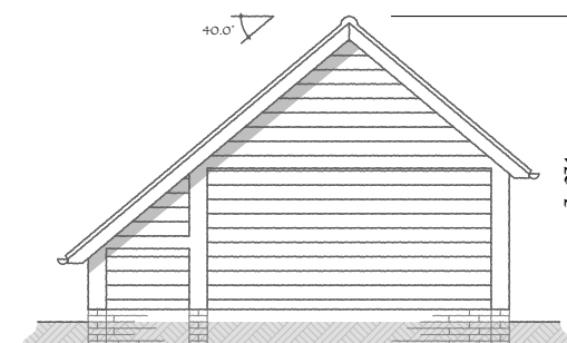
LEFT ELEVATION
