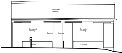
EXISTING ELEVATION [NORTH] 1:200 @ A3
