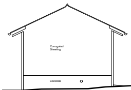
EXISTING ELEVATION [EAST] 1:200 @ A3
