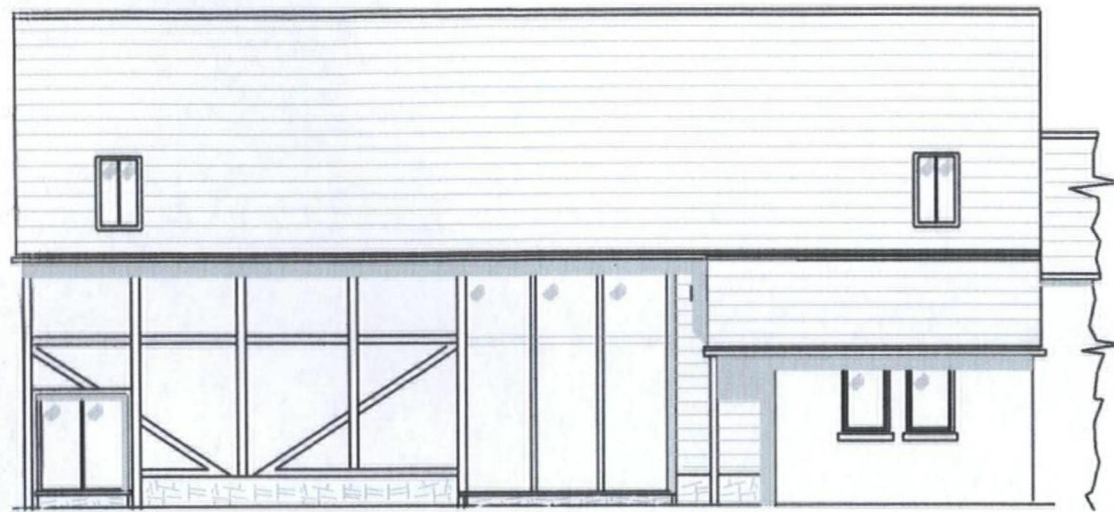
EAST ELEVATION
