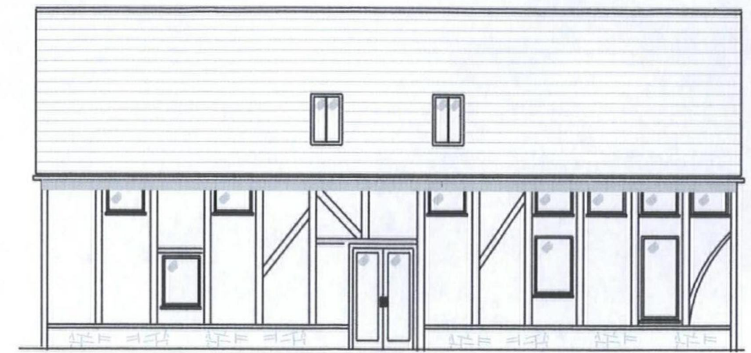
WEST ELEVATION
