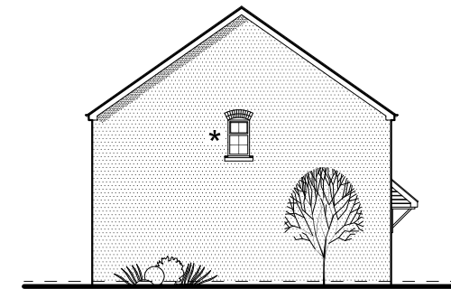
Side Elevation
