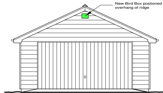
North Elevation
