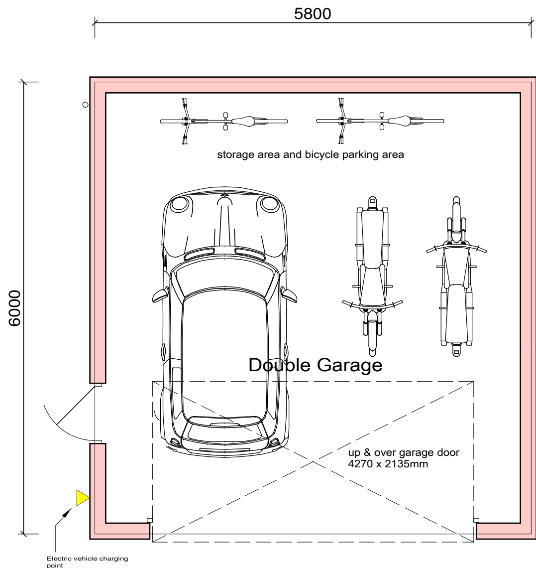
Floor Plan
