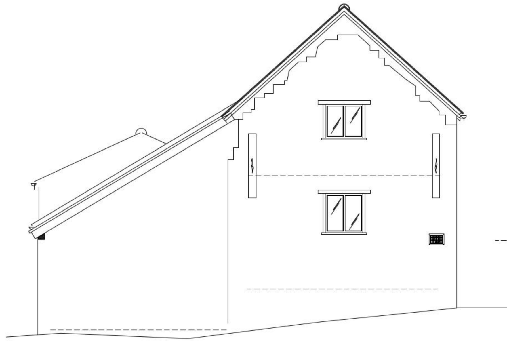
Proposed End Elevation North East Elevation
