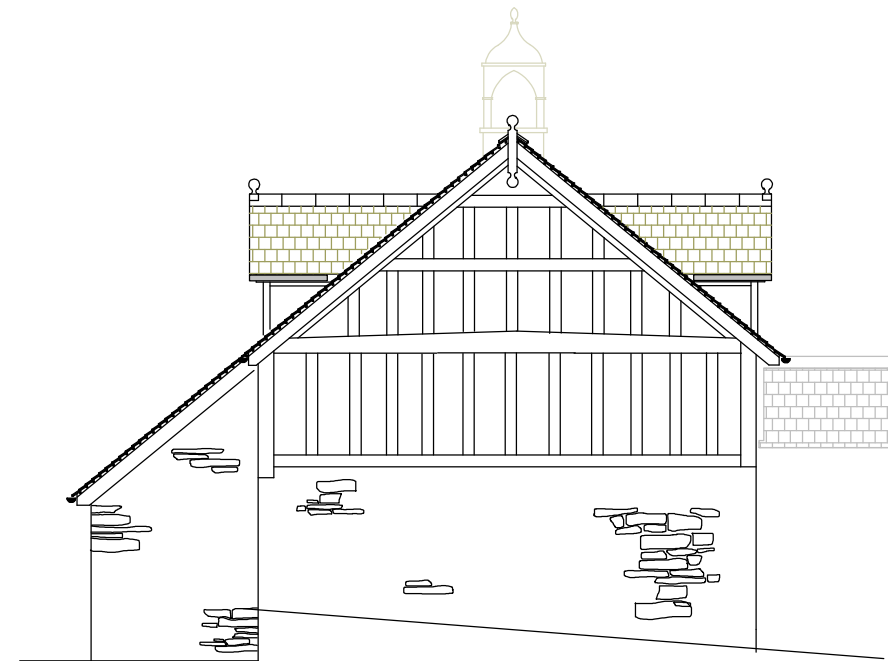
SOUTH ELEVATION
