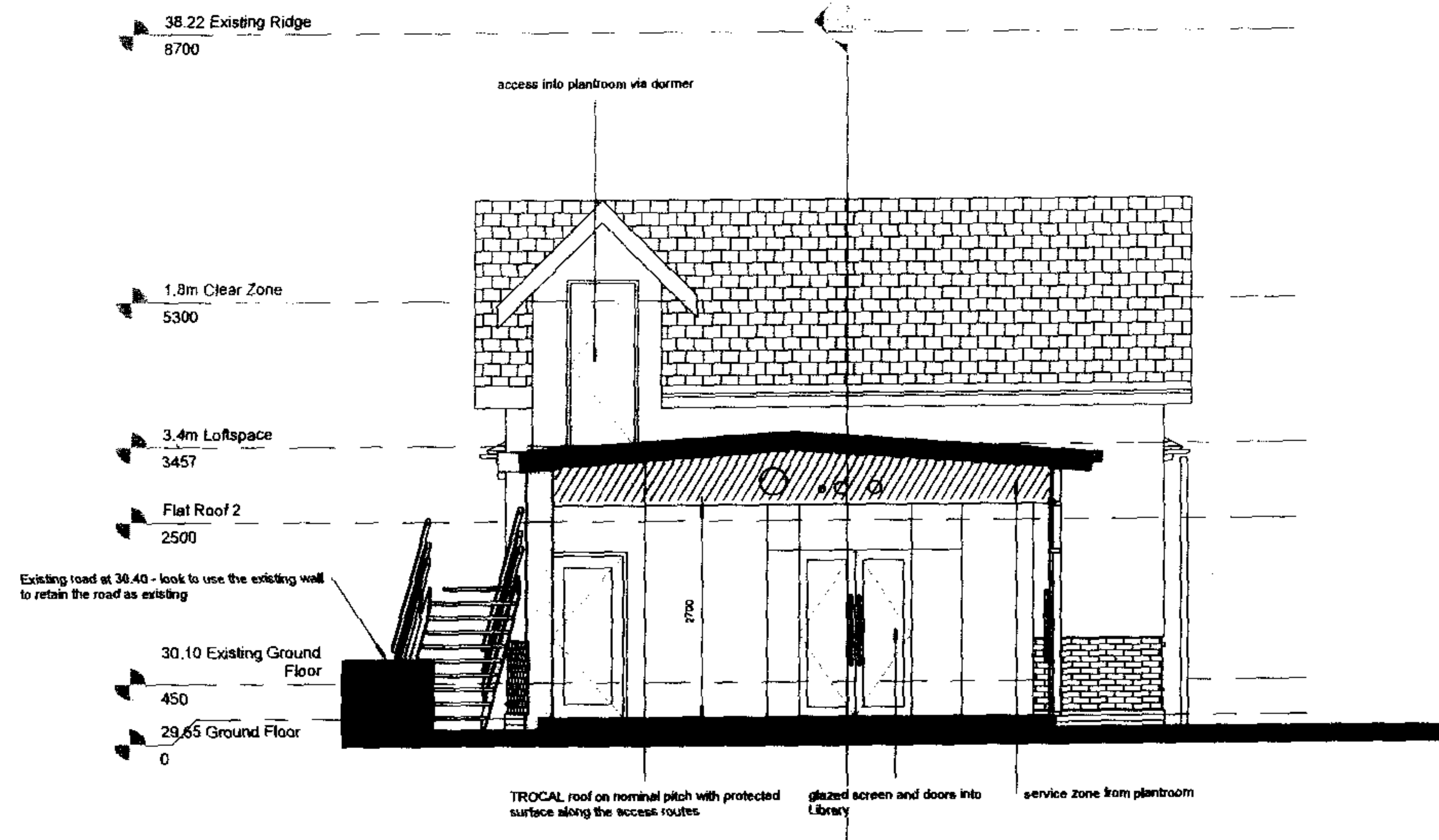
2 Section Through the Entrance 1:50
