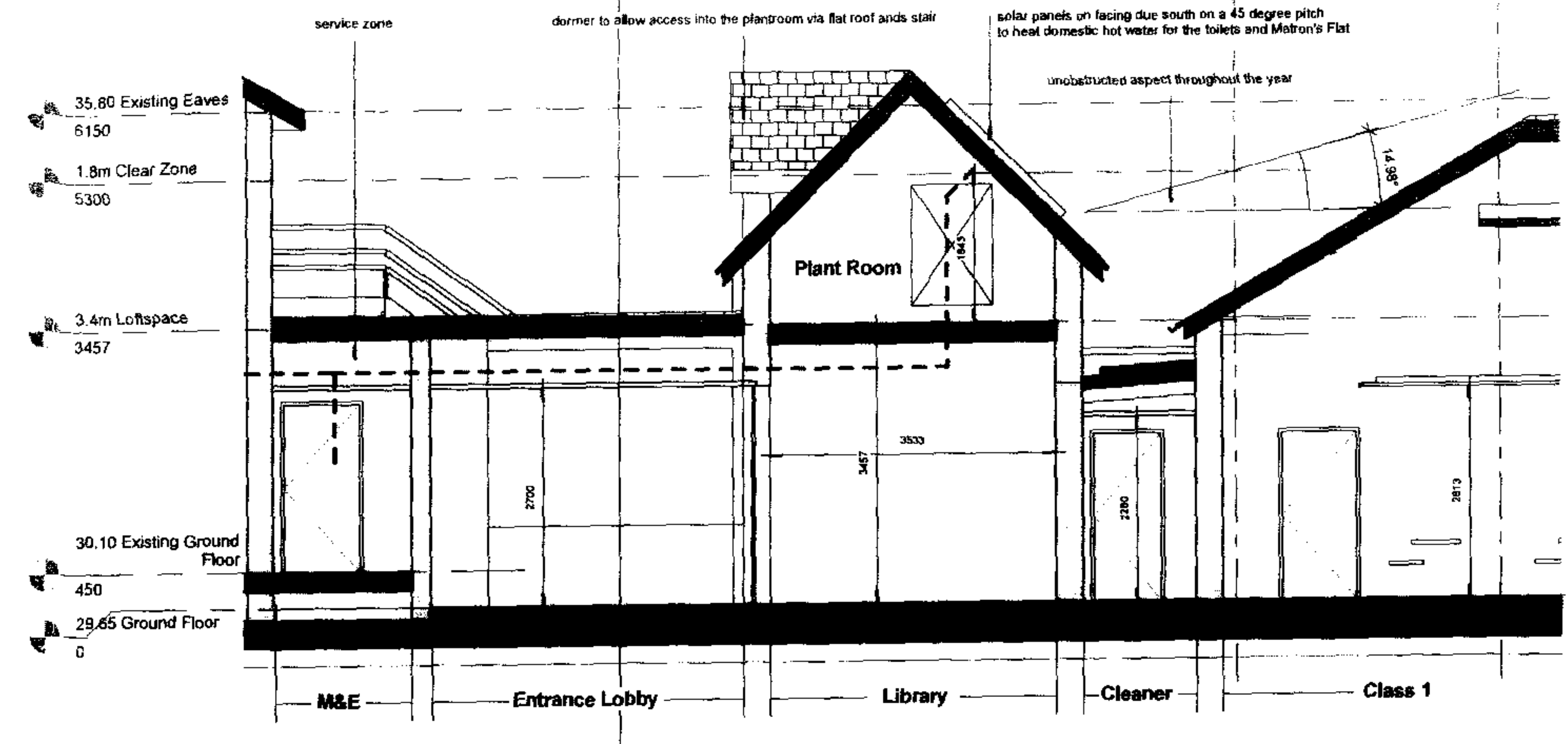
3 Section AA 1:50
