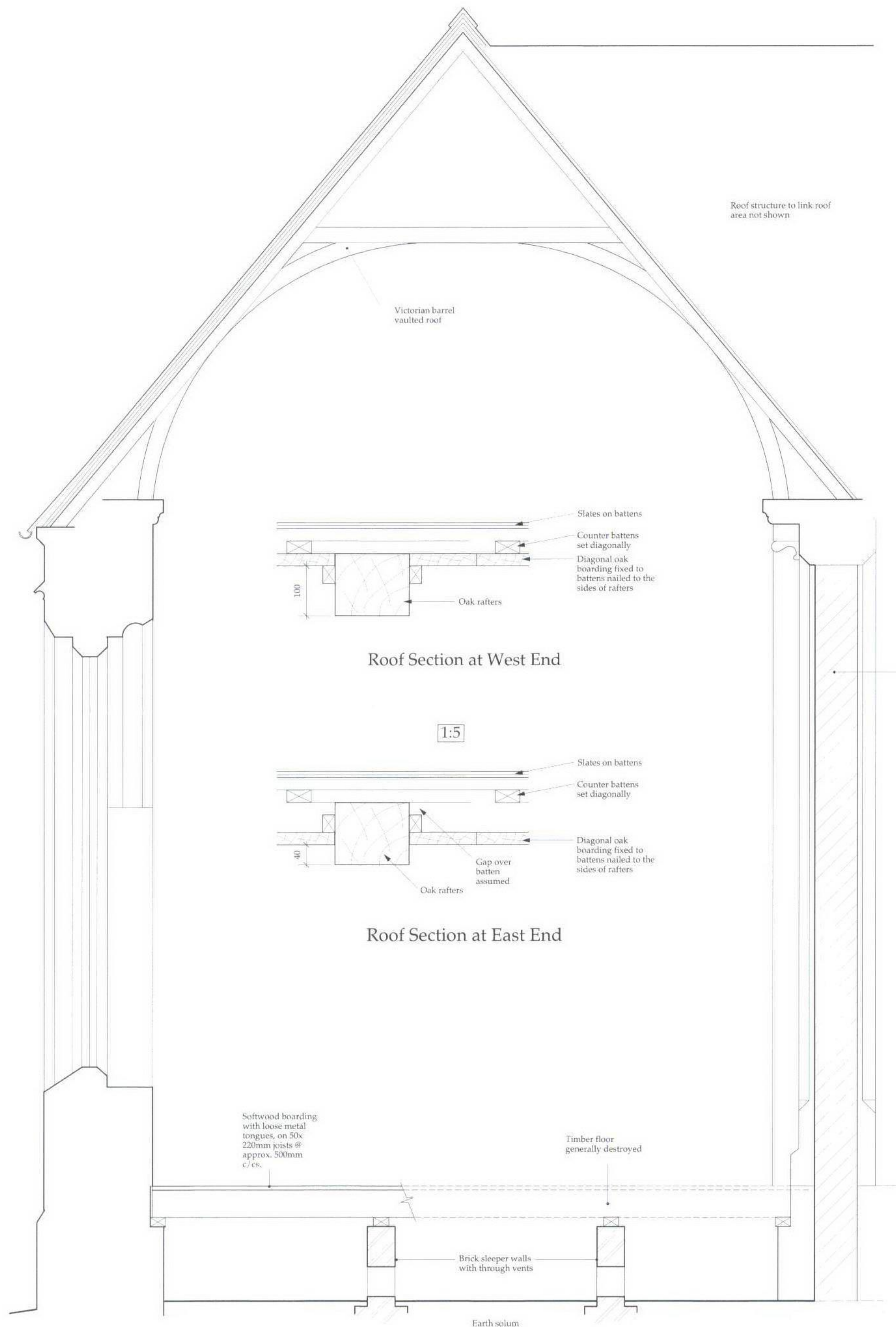
Section at West End
