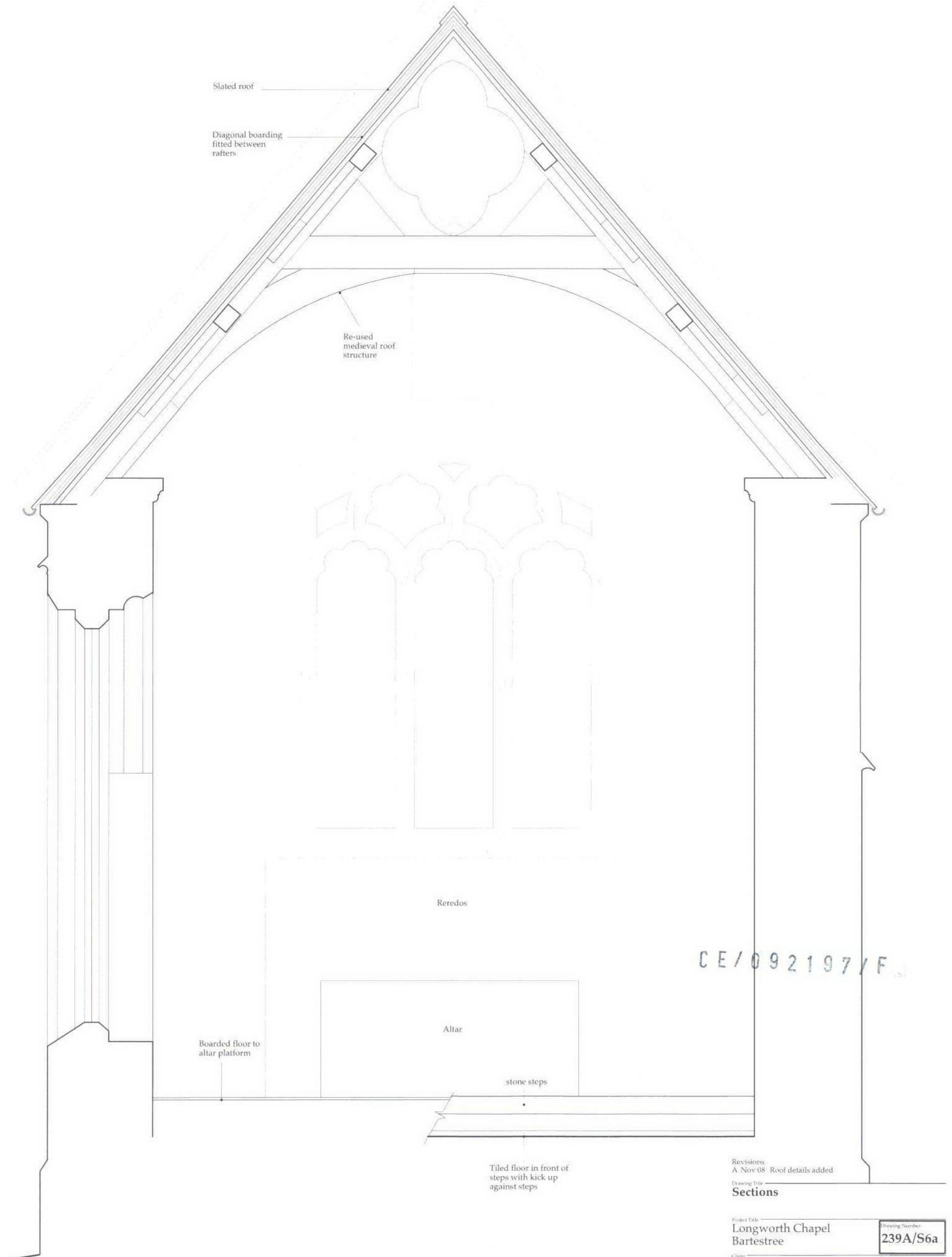
Section at East End
