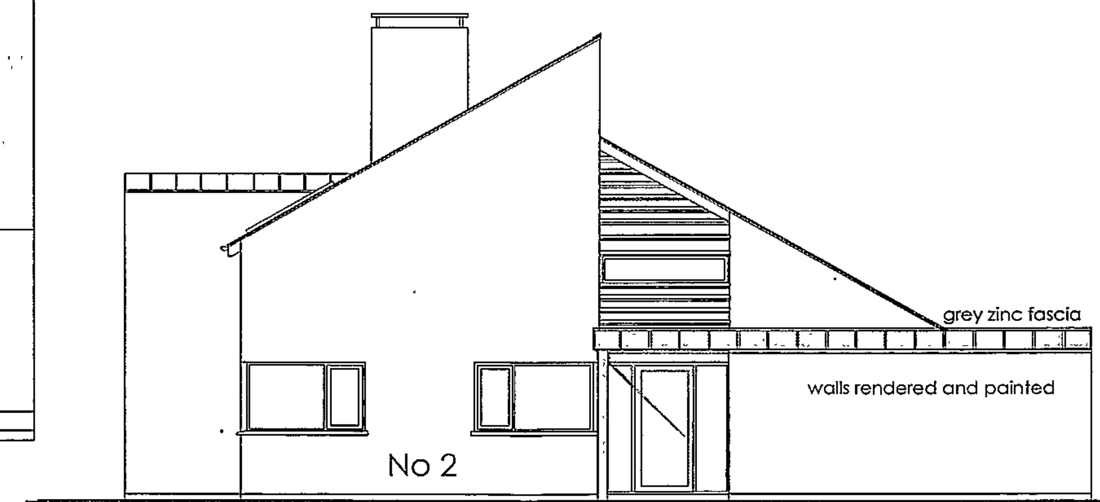
Side Elevation unit 1
