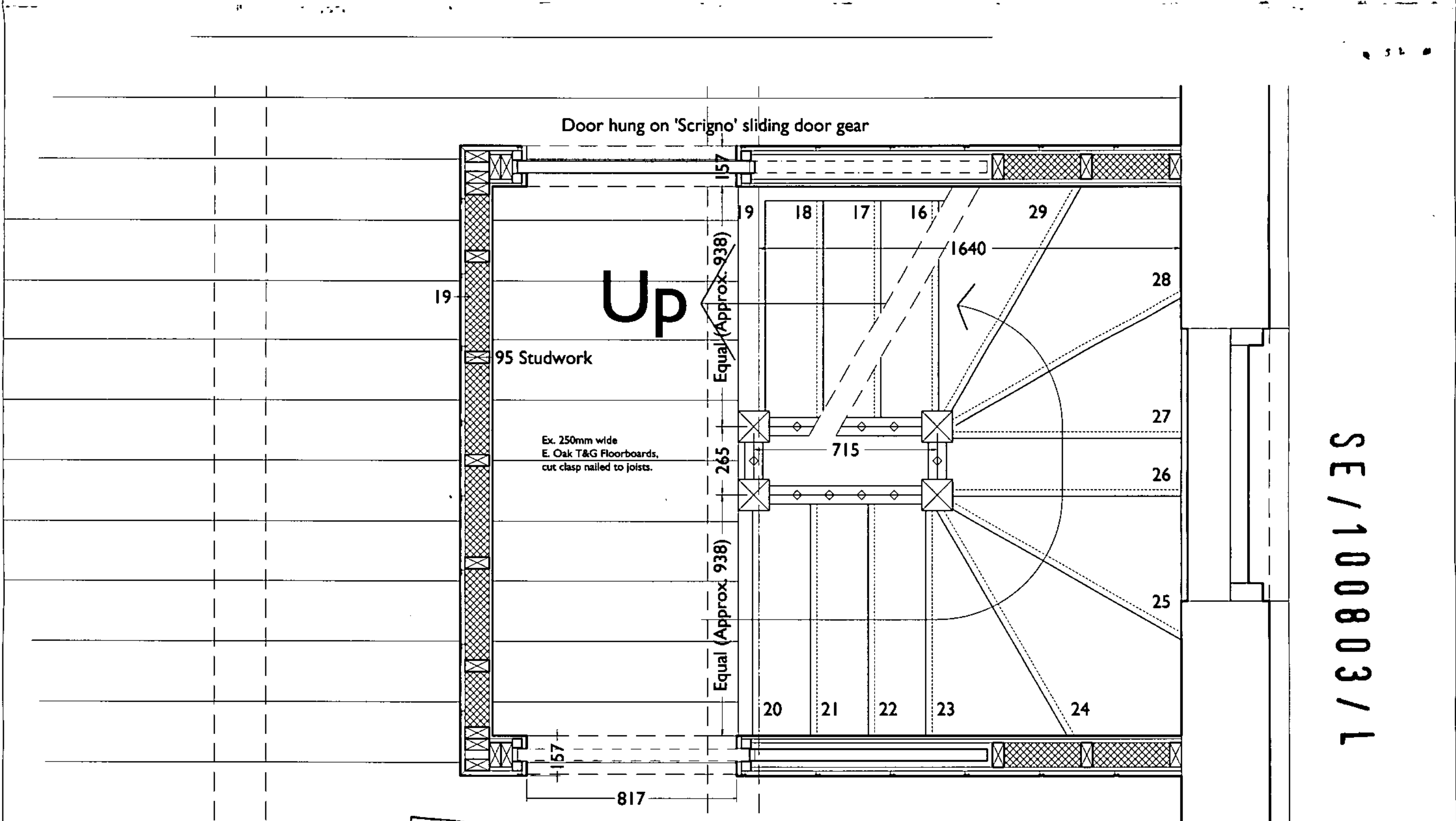
Proposed Staircase Plan Detail - First Floor
