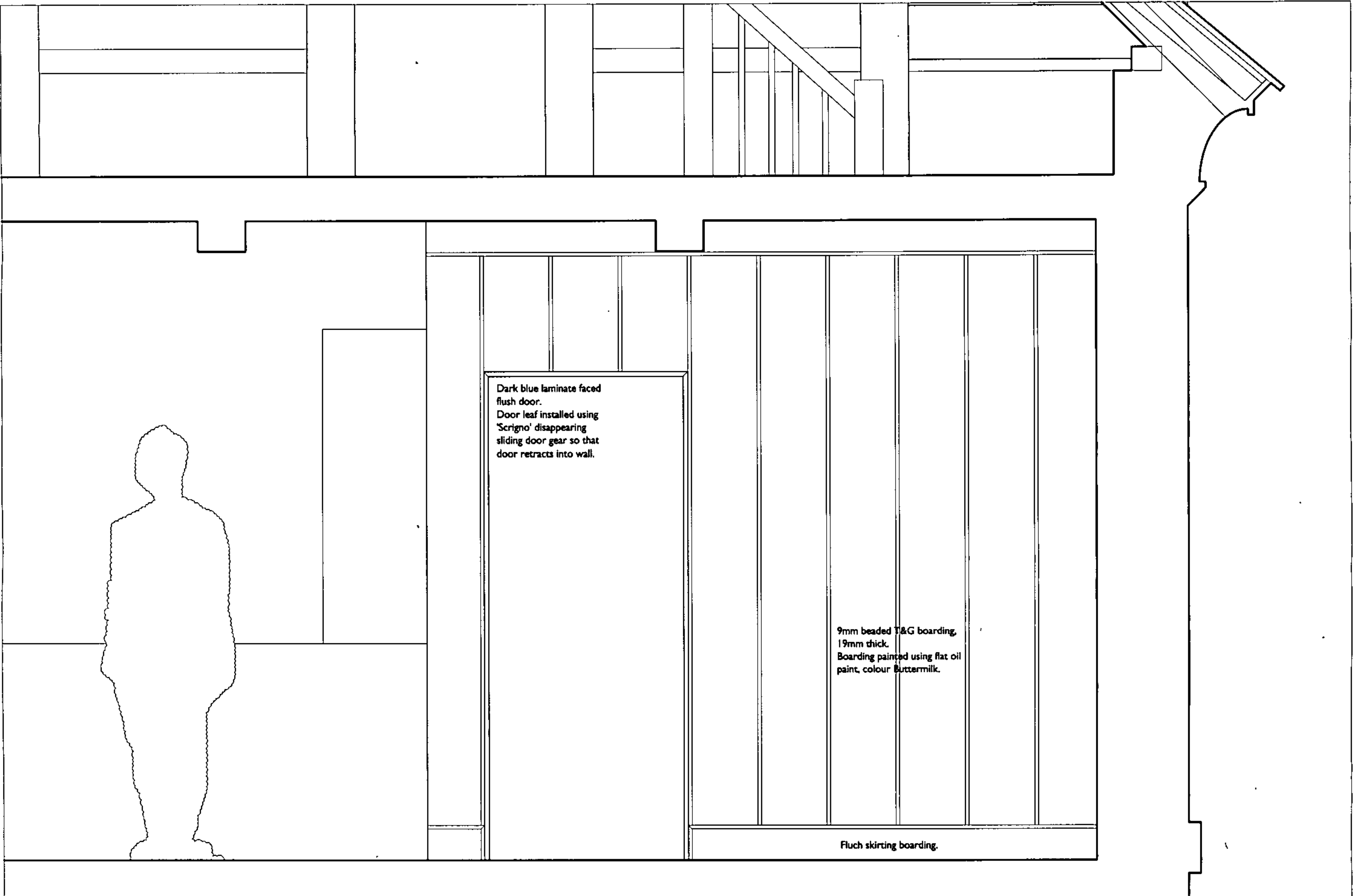
Proposed Staircase Section Detail - First Floor
