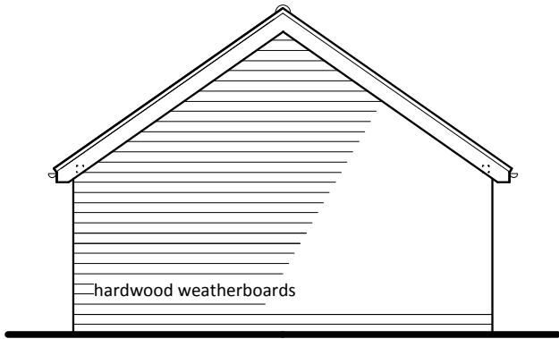
SOUTH-WEST ELEVATION
