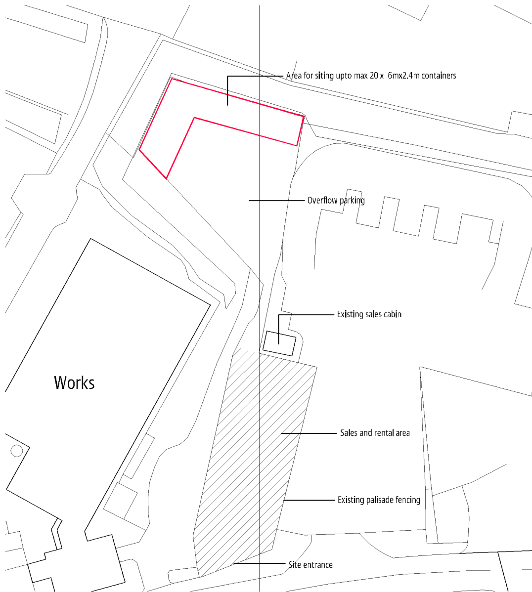
SITE PLAN 1:500 area 0.14Ha
