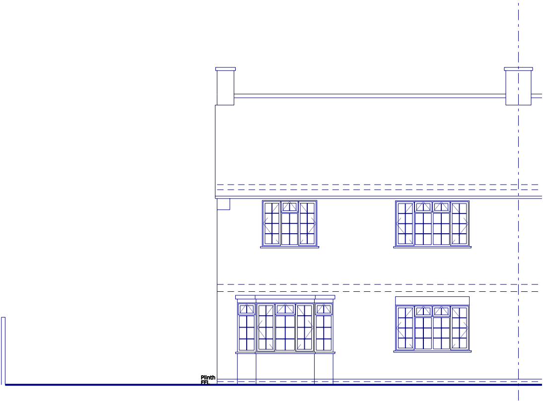
SOUTH-WEST ELEVATION
