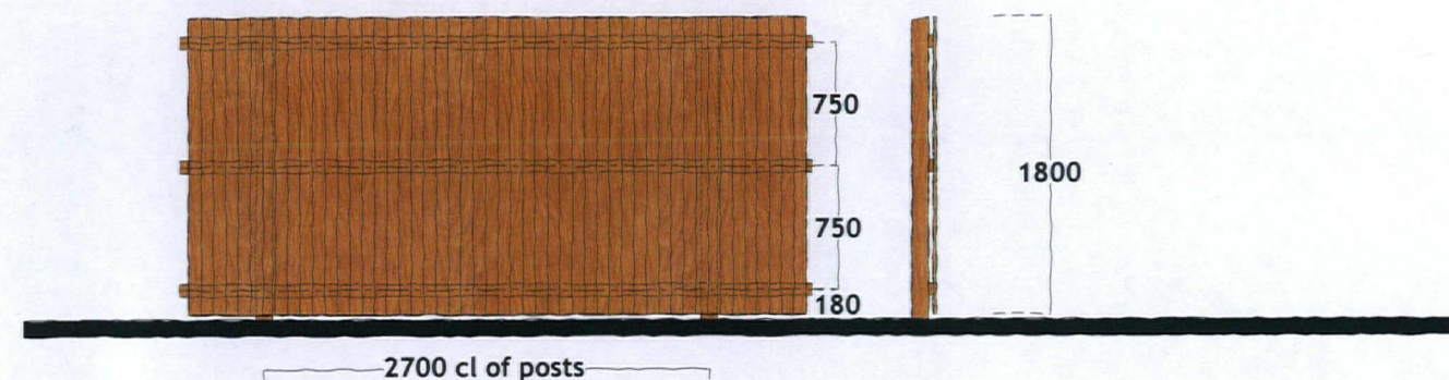
1800mm high Timber Fence.
