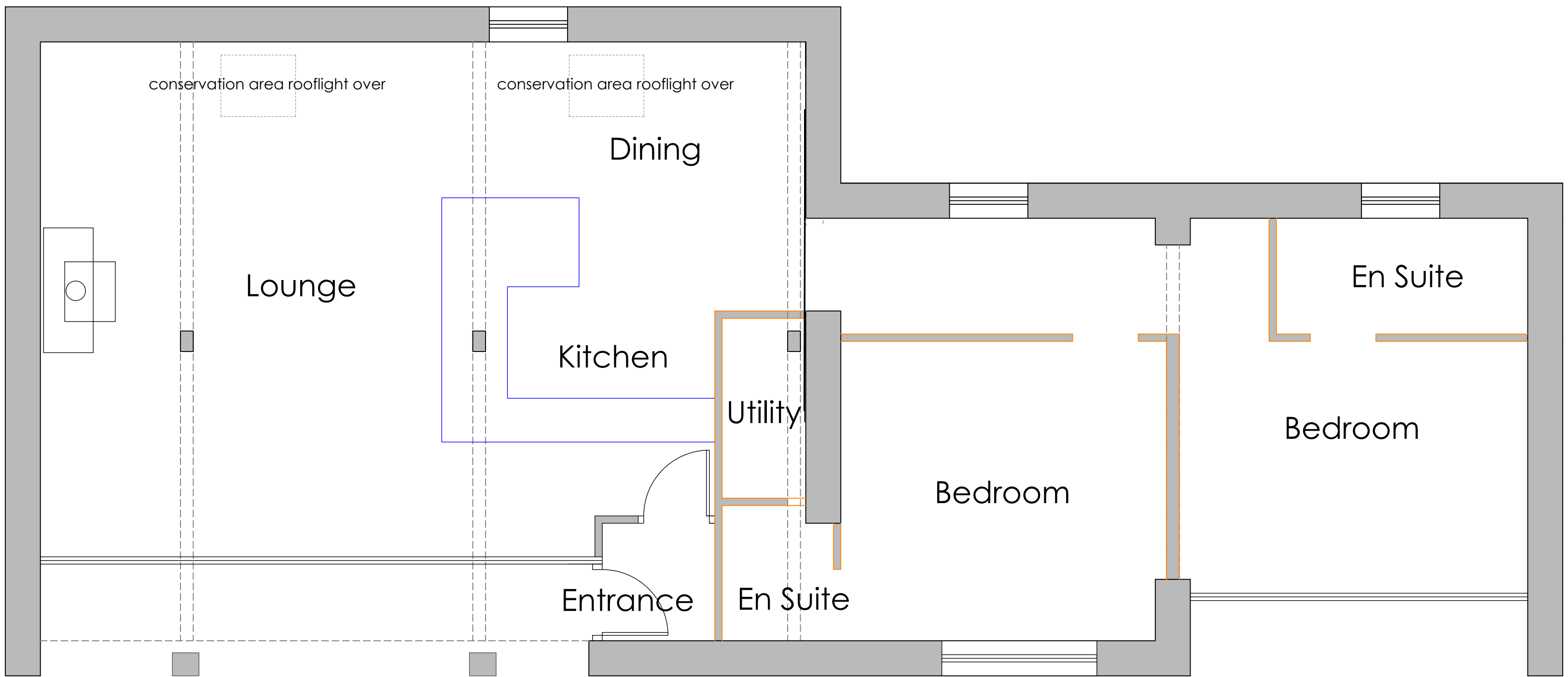
Ground Floor Plan as Proposed
