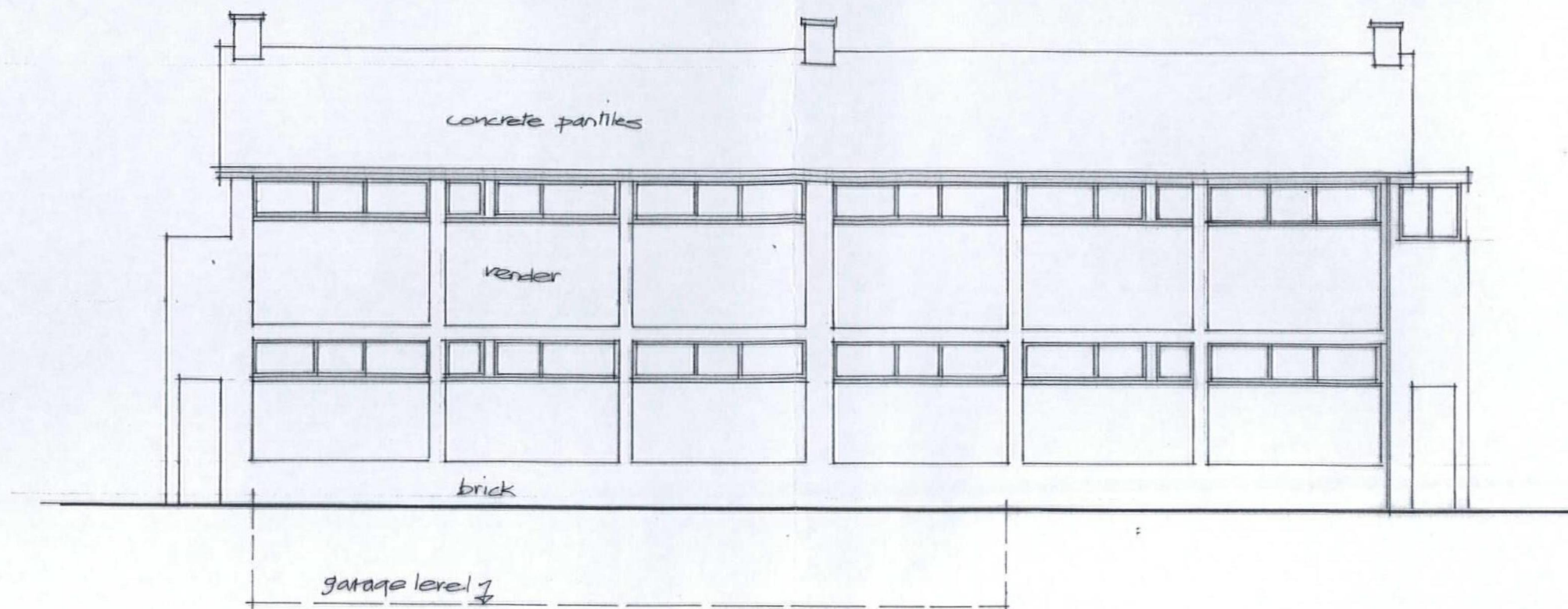
Rear Elevation (South East)
