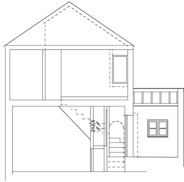
SECTION TO SHOW PROPOSED STAIR
