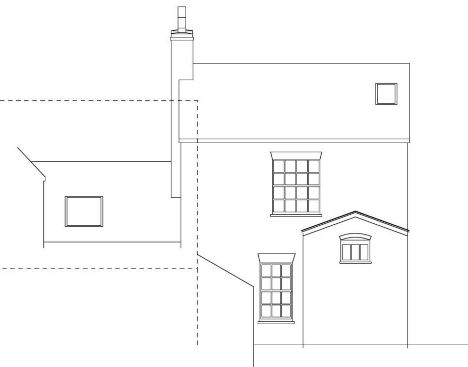
PROPOSED N E ELEVATION WITH DOUBLE PITCHED ROOF TO BATHROOM
