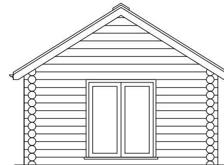
East Elevation (Side)
