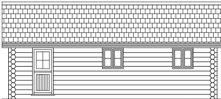
North Elevation (Front)
