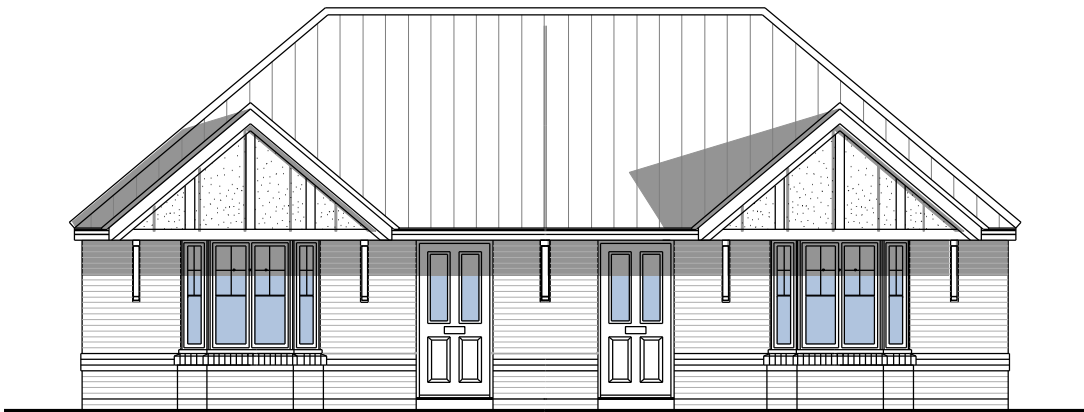
FRONT ELEVATION - SEMI DETACHED
