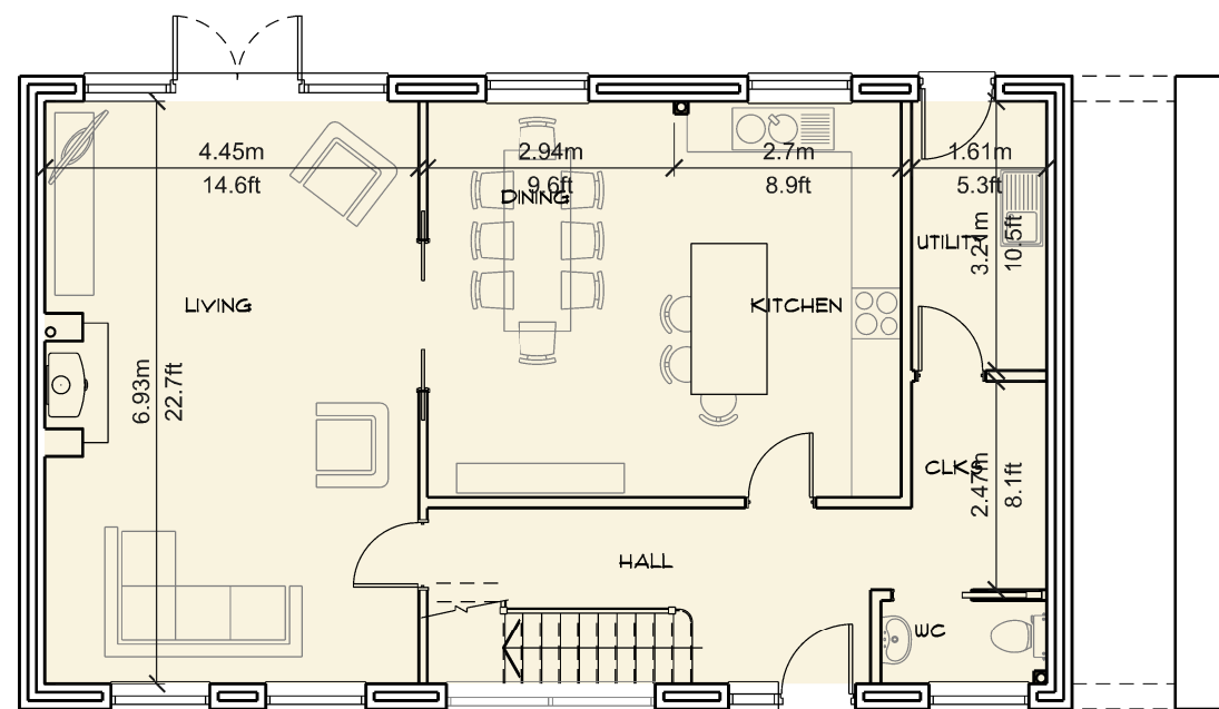
GROUND FLOOR PLAN AREA - 82.6 SQ. M - 888.6 SQ. ' TOTAL AREA - 176 SQ.M - 1,891 SQ.FT
