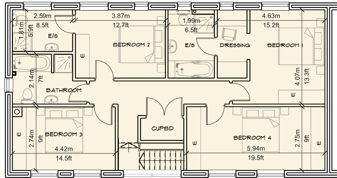
FIRST FLOOR PLAN AREA - 93.1 SQ. M - 1002.4 SQ. '
